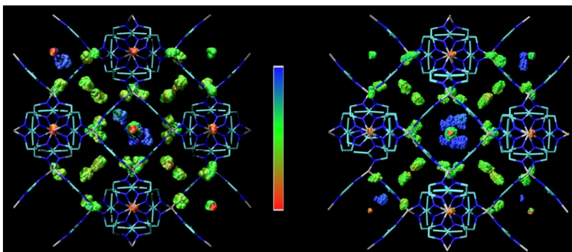
Figure 6: (a) Heat map of N_2 in ZIF-8-HP. (b) Heat map of O_2 in ZIF-8-HP. Points are centre of masses of diatomic molecules and the colour represents the framework – fluid interaction energy. Red corresponds to low energy (strong interaction) and blue to high energy (weak interaction).
