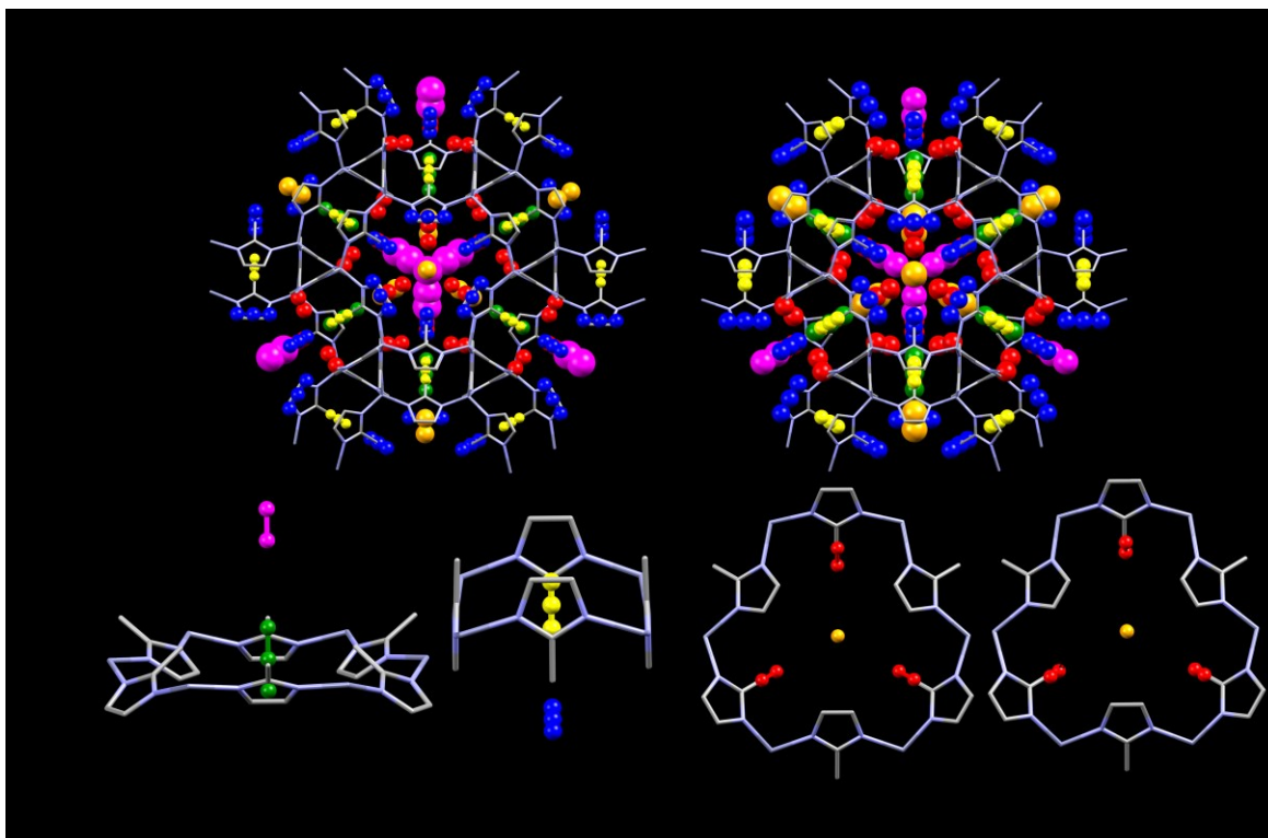
Figure 5: Experimentally-derived unit cell of ZIF-8-HP with (a) adsorbed N_2 molecules at 3.25 GPa, and (b) adsorbed O_2 molecules at 1.20 GPa. In (a) and (b) guest shown as ellipsoids (50% probability) and each colour represents symmetry independent adsorption sites. (c) 6MR window with sites O_2 -1 and O_2 -6 (d) 4MR window with sites O_2 -3 and O_2 -4 (e). 6MR window with O_2 -2 and O_2 -5 showing O_2(1) - O_2(2) -C3 angle of 130^\circ , (f) 6MR window with N_2 -2 and N_2 -5, showing N_2(1) - N_2(2) -C3 angle of 150^\circ . Note as (c) and (d) N_2 analogues are similar, their structures are not represented here.
