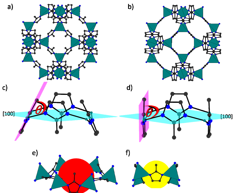
Figure 1: a) ZIF-8-AP with 4MR window in the faces and 6MR windows in the body diagonal. (b) ZIF-8-HP with mIm linkers rotated by 30° compared to the AP structure (c) 4MR window showing the opening angle of 68° for ZIF-8-AP, (d) 4MR window showing the opening angle of 89° for ZIF-8-HP, (e) 6MR window with pore diameter of 3.0 Å and (f) 4MR window with pore diameter of 0.8 Å.
