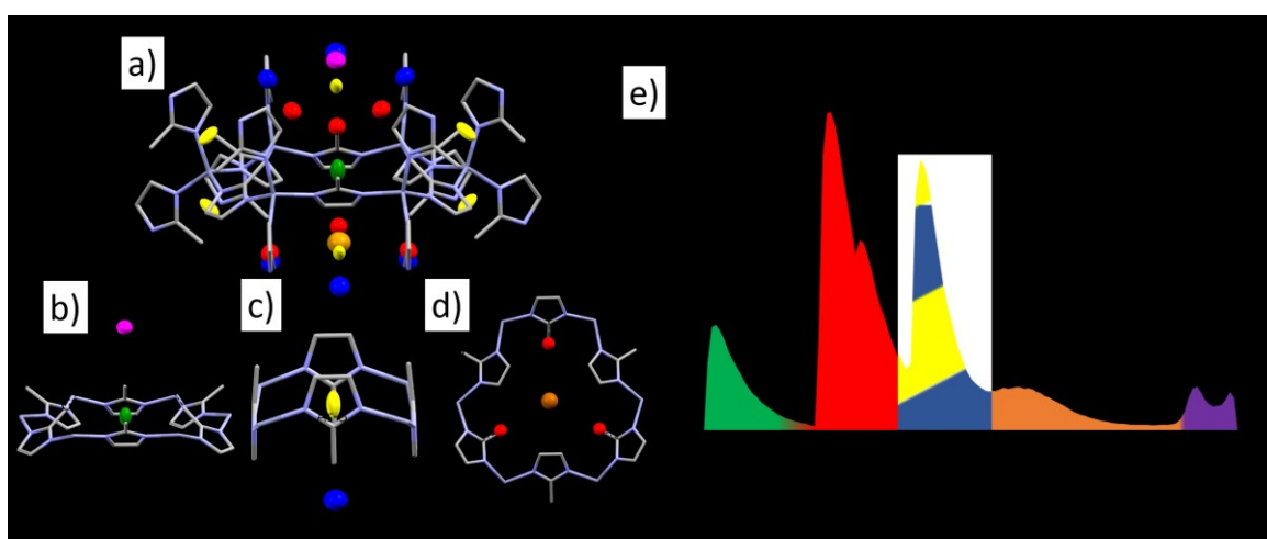
Figure 4: a) Ar adsorption sites in ZIF-8 at 1.20 GPa as shown on a 6MR window for Ar-1 (green), Ar-2 (red), Ar-3 (yellow), Ar-4 (dark blue), Ar-5 (orange), Ar-6 (magenta). Short contacts for (b) Ar-6 with the methyl C-atom (C1) and (c) Ar-4 with the imidazole C-atom (C2) and (d) Ar-5 (with C2) are drawn as black dotted lines and discussed in the text. (e) Histograms showing the frequency of guest-framework interaction energies at 100 kPa of guest during GCMC simulation in ZIF-8-Ar using ZIF-8-HP. Sections are coloured according to the adsorption sites Ar-1 to Ar-6 (Ar-4 and Ar-5 cover the same energy range). Colour scheme; Zn (light grey), N (light blue) and C (grey). Hydrogen atoms have been omitted for clarity, ellipsoids for Ar-atoms are drawn at 50 % probability, whilst the ZIF-8 framework is drawn as capped sticks.
