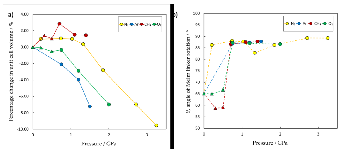
Figure 2: (a) Change in unit cell volume of ZIF-8 with pressure for N 2 (yellow), CH 4 (red), Argon (blue), O 2 (green); (b) Change in angle of rotation of Melm linker, \theta , in ZIF-8 upon increasing pressure for N 2 (yellow), O 2 (green), Ar (blue) and CH 4 (red). Triangles and circles indicate ZIF-8-AP and ZIF-8-HP phases, respectively.
