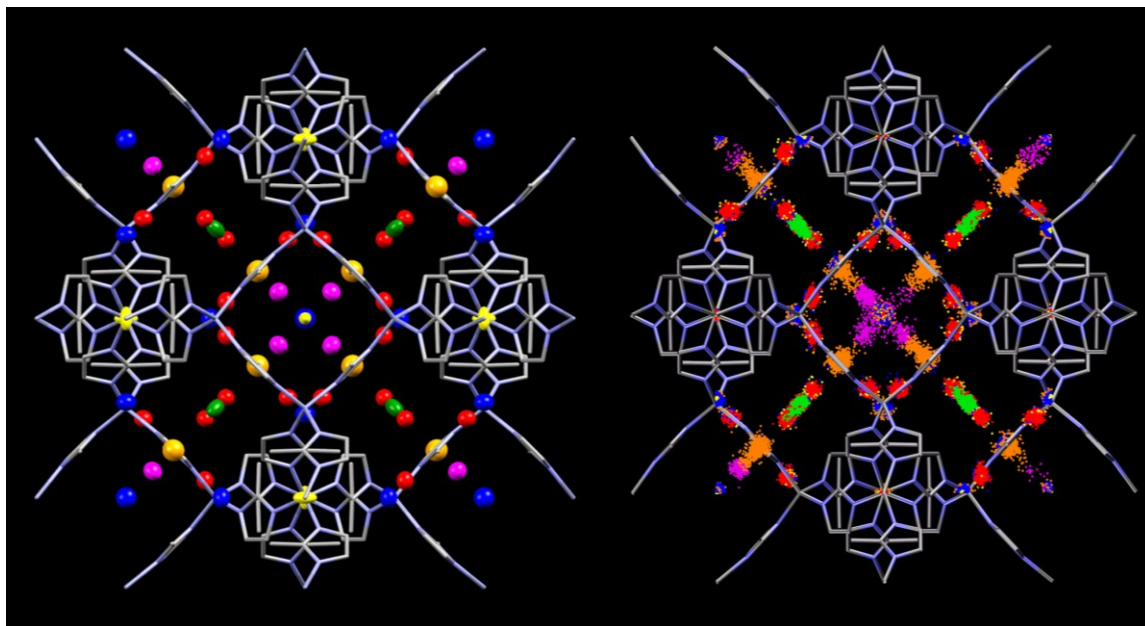
Figure 3: Comparison of Ar adsorption sites in ZIF-8-HP from (a) 1.20 GPa (298 K) crystal structure and (b) GCMC simulations at 100 kPa (at 83 K) of Ar. Colour scheme; Zn (light grey), N (light blue) and C (grey). Hydrogen atoms have been omitted for clarity. In (a) and (b) framework atoms are drawn as capped sticks, while Ar atoms are coloured according to the six symmetry independent sites. In (a) Ar atoms are drawn with anisotropic displacement parameters (50 % probability), while in (b) Ar atoms are shown as the binned positions with their relative energies from the GCMC simulation.
