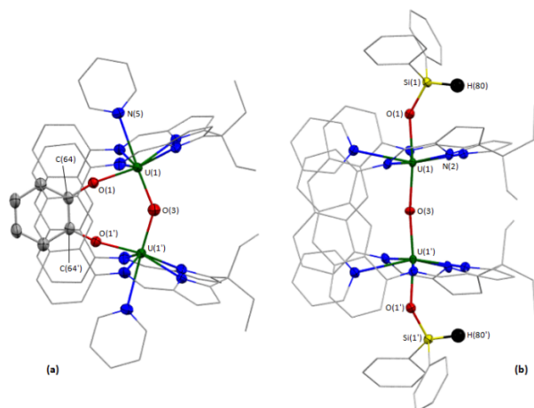
FIGURE 1. Solid-state structures of 2-2-toluene (a) and 3-THF (b). Displacement ellipsoids are drawn with 50 % probability, and carbon atoms of \text{L}^{\text{A}} and U-coordinated solvent molecules drawn wireframe. For clarity, hydrogen atoms, lattice solvent, and lower-fractional occupancy disorder components of the OBpin ligand (B(1)), and \text{L}^{\text{A}} ethyl groups of 2-2-toluene are omitted.
