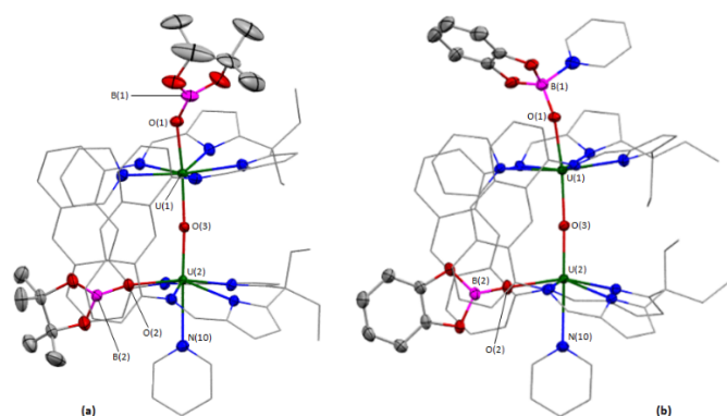
FIGURE 1. Solid-state structures of 2-2-toluene (a) and 3-THF (b). Displacement ellipsoids are drawn with 50 % probability, and carbon atoms of \text{L}^{\text{A}} and U-coordinated solvent molecules drawn wireframe. For clarity, hydrogen atoms, lattice solvent, and lower-fractional occupancy disorder components of the OBpin ligand (B(1)), and \text{L}^{\text{A}} ethyl groups of 2-2-toluene are omitted.
