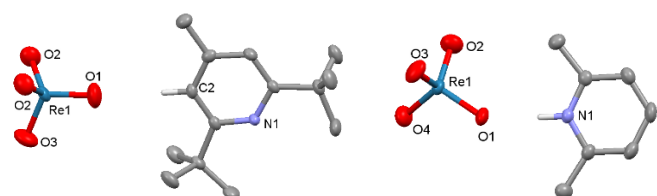
Figure 1. Solid-state structures of 2 (left) and 3 (right). For clarity, all hydrogen atoms, except those involved in hydrogen-bonding, are omitted (displacement ellipsoids are drawn at 50% probability). Selected bond lengths (Å): 2 : Re1-O1 1.703(4); Re1-O2 1.723(4); Re1-O3 1.703(4); C2---O1 3.312. 3 : Re1-O1 1.736(2); Re1-O2 1.714(2); Re1-O3 1.710(2); Re1-O4 1.716(2); N1---O1 2.754.
