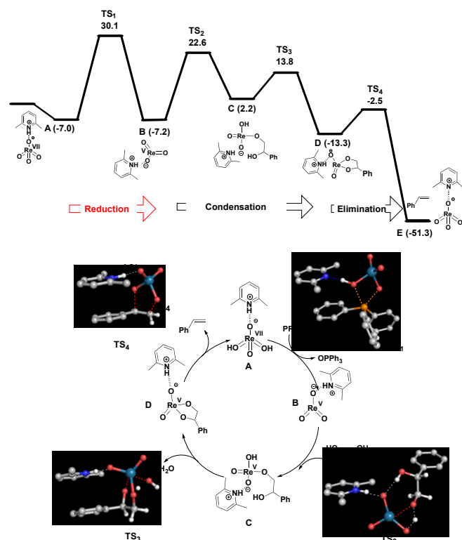
Figure 2. Structures and relative free energies ( \Delta G , in \text{kcal mol}^{-1} ; selected distances in \text{\AA} ) of stationary points involved in the catalytic cycle for the DODH reaction of styrene diol by 3 . Energy values were calculated at the SMD( \text{CHCl}_3 )/B3LYP-D3(BJ)/Def2TZVP//B3LYP-D3(BJ)/6-31G+(d) level of theory relative to the separated species.
