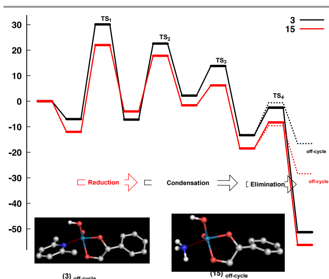
Figure 3. Comparison of the structures and relative free energies ( \Delta G , in kcal mol ^{-1} ) for the catalytic DODH reaction of styrene diol by 3 (black) and 15 (red) proceeding via reduction, condensation and elimination (Path A). Energy values were calculated at the SMD(CHCl _3 )B3LYP-D3(BJ)/Def2TZVP//B3LYP-D3(BJ)/6-31G+(d) level of theory relative to the separated species. The production of off-cycle products as a result of proton-shuttling and base coordination is shown.
