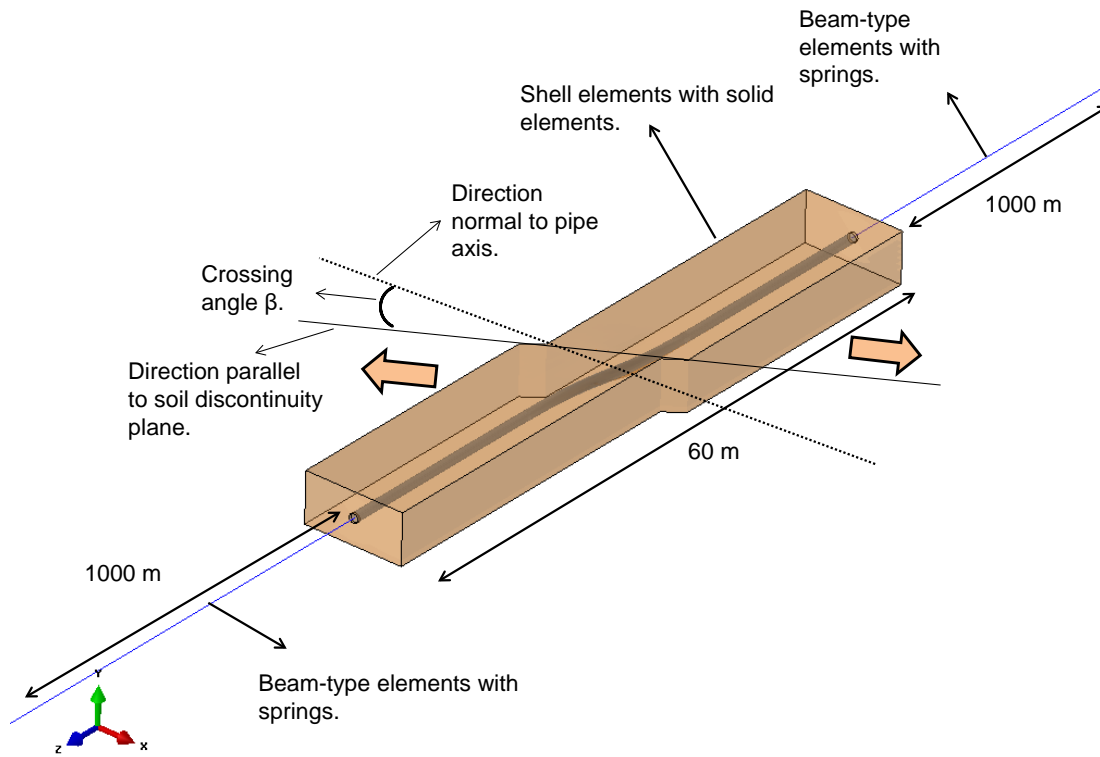
Figure 10. Pipeline configuration in a horizontal (strike-slip) seismic fault crossing; crossing angle \beta is measured with respect to the direction normal to the pipeline axis.
