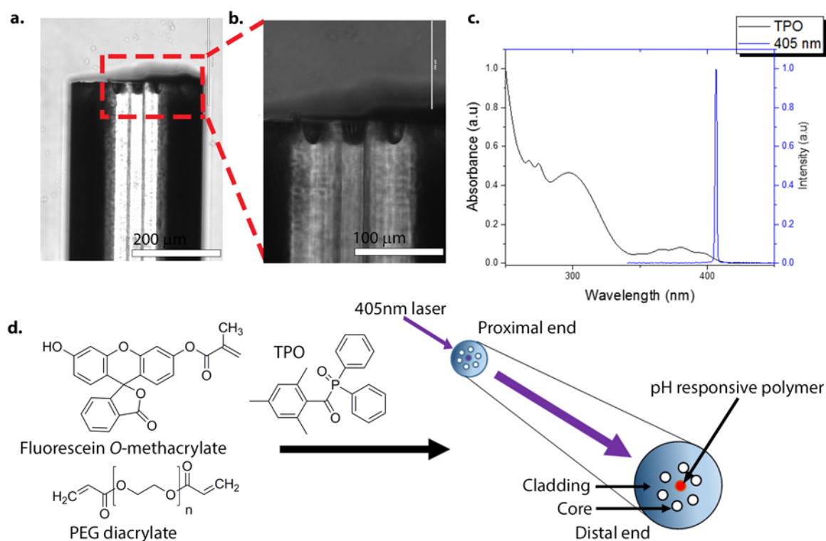
Figure 1. (a) - (b) The side view images of an etched optical fibre. The pit's depth was approximately 30 \mu m. The distal end of the etched optical fibre was HF-etched and silanized in 3-(trimethoxysilyl)propyl methacrylate (TMSPMA) (20% in acetone) to introduce acrylate groups onto the distal surface of the pit. (c) The absorbance spectrum of diphenyl(2,4,6-trimethylbenzoyl)phosphine oxide (TPO) (2.5 mM in ethanol) (black line), and the 405 nm laser spectrum (blue line). TPO absorbs in the UV range up to about 425 nm, and although not optimal, it allowed sufficient excitation and radical generation by TPO (it is worth noting that the light source used by dentist with this initiator are typically in the wavelength range of circa 380 to 520 nm (dual peak LED)). 23 (d) The method used for photo-polymerisation at the distal end of the optical fibre. Only seven (of the 19) cores of the optical fibre are shown for clarity. The laser was coupled to a specific core of the fibre via an XYZ translational stage. Once coupled, the distal end was dipped into the polymerisation solution containing fluorescein O -methacrylate (10 mol%), PEG-diacrylate (87 mol%), and TPO (3 mol%).
