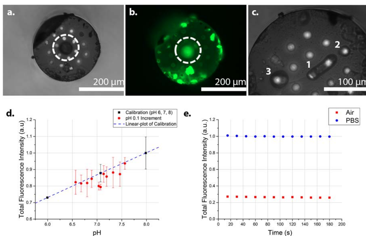
Figure 2. Photo-polymerisation of fluorescein O -methacrylate and PEG diacrylate at the end of the optical fibre. (a) Image of the distal surface of an optical fibre, containing one fluorescein polymer core in the middle core (white circle) (b) The polymer fluoresced green under 488 nm excitation (white circle). (c) The distal surface of an optical fibre showing three fluorescein polymers (labelled 1, 2, and 3) at different cores. The polymers were grown individually, with defined core-to-core photo-polymerisation, with fresh polymerisation solution used for every polymerisation. The polymer labelled 1 distorted during photo-polymerisation thus extending to the nearest core. The polymers generated filled the depth of the pits, thus giving polymer features of approximately 30 \mu m in depth (d) The integrated fluorescence intensity of the fluorescein O -methacrylate-based sensor at 0.1 pH increments from pH 6.6 to 7.6 (Figure S4), with the three calibration points (pH 6, 7, and 8) ( n = 2 ) ( R^2 = 0.99 ). The fluorescence measurements of 0.1 pH increments were in random order, while the calibration points were in ascending order. (e) The integrated fluorescence intensity of the fluorescein polymer with continuous illumination for 180 seconds in PBS (pH 7.4) (blue circles) and in air (red squares), showing the photo-stability of the sensor. Very little evidence of photo-bleaching was observed. In a realistic usage environment, discrete measurements would be performed, rather than the continuous illumination demonstrated here (180 seconds continuous exposure). The small variation of the intensity may also be attributed to the intensity fluctuations in the excitation source. All measurements were made in a dark room with excitation wavelength = 485 nm, with the laser operating at 1.0 \mu W.
