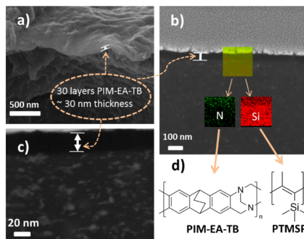
Figure 4. Electron microscopy images of the composite membrane PTMSP/PIM 30 with a thickness (measured in 15 different points along the sample) of 30.5±2 nm of PIM-EA-TB(H 2 ) layer (30 LS films deposited onto PTMSP): a) SEM cross-section, b) focused ion beam with an inset including an EDX mapping (N in green and Si in red), c) TEM image from a lamella extracted from the sample specimen and d) chemical structure of the polymers forming the composite membrane.
