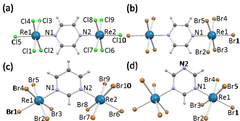
Figure 1. The structures of 1-4 (a-d). Colour code: Re, cyan; Br, brown; Cl, green; C, grey; N, blue; H, white.
