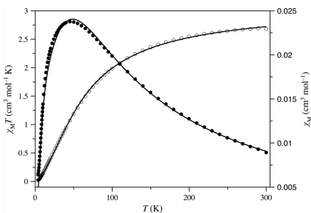
Figure 2. Thermal dependence of \chi_M T (○) and \chi_M (●) under an applied dc field of 0.1 T for 1 . The solid line is the best-fit curve (see text).
