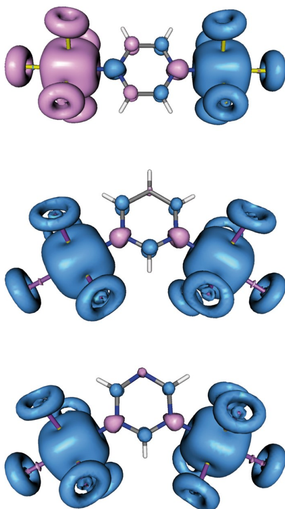
Figure 7. Spin density plots for the ground spin states in (representative) 1 , 3 and 4a . The isodensity surfaces correspond to a cut-off value of 0.002 \text{ e bohr}^{-3} . Blue and magenta isosurfaces represent positive and negative regions of spin density, respectively.
