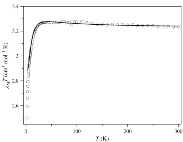
Figure 4. Thermal dependence of \chi_M T (○) under an applied dc field of 0.1 T for 3 . The solid line is the best-fit curve (see text).
