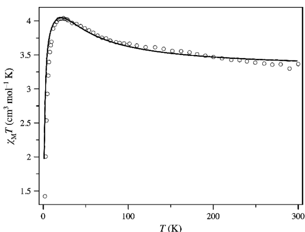
Figure 5. Thermal dependence of \chi_M T (O) under an applied dc field of 0.1 T for 4 . The solid line is the best-fit curve (see text).
