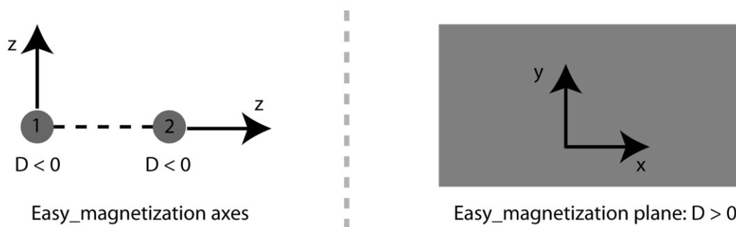
Figure 9. Scheme to visualize how two perpendicular easy-magnetization axes turn into an easy-magnetization plane.
