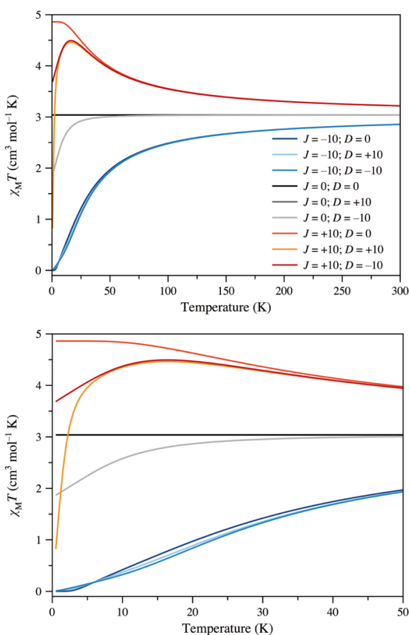
Figure 6. Theoretical thermal dependence of the \chi_M T product for a \text{Re}^{\text{IV}}_2 model complex as a function of different J and D values with g = 1.8 . The lower panel highlights the regime in the temperature range 0 – 50 K.
