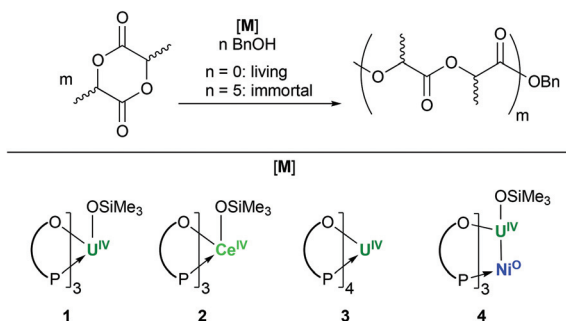
Fig. 1 Summary of ROP of L-lactide studied for the new U^{IV} and Ce^{IV} initiators 1 to 4. The O–P arc is used to represent the OAr^P ligand ( OAr^P = OC_6H_2-6-tBu-4-Me-2-PPh_2-\kappa^2 O,P ).
