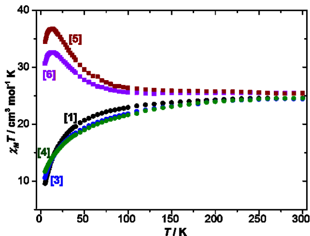
Figure 9. Plot of \chi_M T versus T for complexes 1 and 3-6 measured in the T = 300 - 2 K temperature range in an applied magnetic field of B = 0.1 T.
