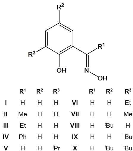
Figure 2. Ten SaoH 2 -based co-ligands explored as candidates for complementary cluster formation with TBC[4].
