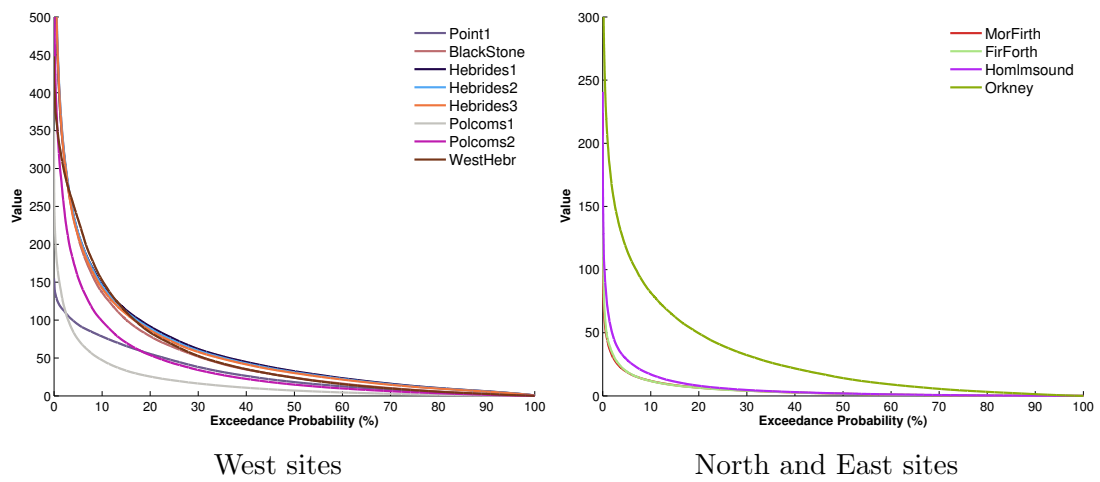
Figure 9.: Exceedance Probability, x-axis in the % probability and y-axis P_{wave} in kW/m
