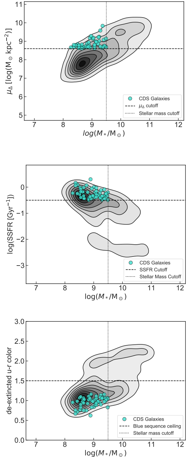
Figure 2. Selection of low- z CDS galaxies with M_{*} < 10^{9.5} M_{\odot} . Top: Selected using the \mu_{\Delta} parameter as a surrogate for Hubble type, the compactness of CDS galaxies reflects the intense compaction events that have driven their starbursts. Middle: The selection of \log(\text{SSFR} [\text{Gyr}^{-1}]) > -0.5 , as in the Barro et al. (2013) high-redshift sample, ensures significant starburst activity. Bottom: The SSFR restriction implicitly requires that galaxies fall on the blue sequence, as shown. In all figures hereafter, the grayscale contours represent the 2D kernel density estimate (KDE) of all RESOLVE galaxies above the survey floor described in §2.1.2. The contour levels are drawn to correspond to the 10th, 20th, etc. percentiles of the probability density function. In the top and middle panels, the lowest level contour is suppressed for visual clarity.
