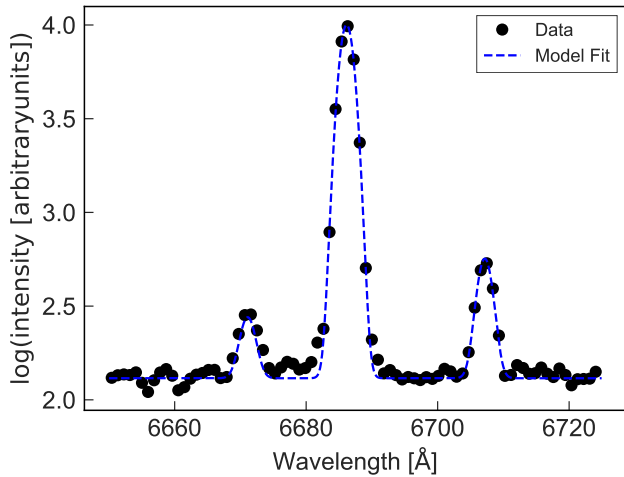
Figure 6. Example spectrum extracted from GMOS IFU data for rf0266 with Gaussian fit. The H \alpha and [NII] emission line data are plotted as black points, with the best-fit triple-Gaussian model overplotted as a dashed blue curve. We obtain greater centroiding accuracy by fitting to the H \alpha and [NII] lines, as opposed to only the H \alpha line. The y-axis is plotted on a log scale for visual clarity.
