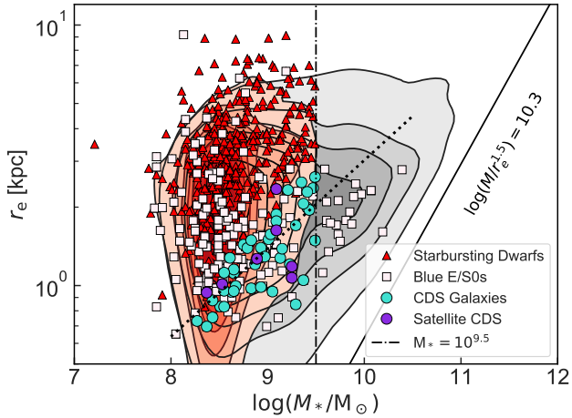
Figure 8. Mass-size diagram for the RESOLVE survey (contours as in Figure 7) with subpopulations marked, revealing the small sizes at fixed mass (high densities) of our CDS sample (centrals as turquoise dots and satellites as purple dots) relative to the general population of high-SSFR dwarfs selected without any \mu_\Delta morphology restriction (red triangles and contours). The low- z CDS mass-size relation (dotted line fit) is tighter and significantly offset toward the edge of the general sample distribution. Some subpopulations such as blue E/S0 galaxies (light pink squares; further discussed in §5) overlap the CDS sample with scatter to even higher (and lower) compactness. Note however that we show blue E/S0s extending above the CDS mass cutoff (vertical black dash-dotted line, see §4.1.2), where the general RESOLVE mass-size distribution also becomes slightly more compact. Notably, no part of the z \sim 0 galaxy population reaches the mass-size relation implied by the surface density selection of Barro et al. (2013), indicated by the solid black line.
