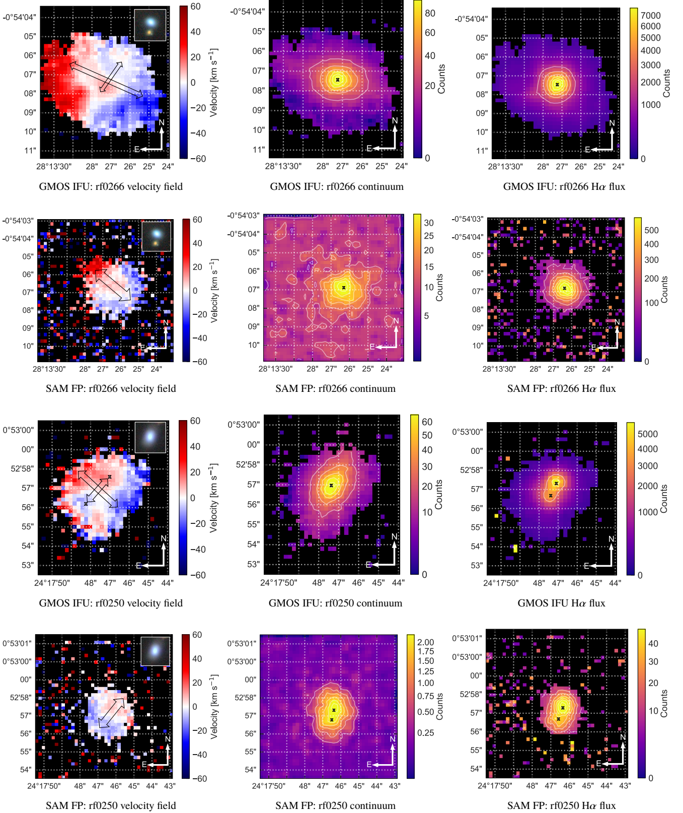
Figure 13. Velocity fields (left column), continuum maps (middle column), and H \alpha flux maps (right column) derived from 3D spectroscopic observations. Nuclei are denoted with an “x” and rotation patterns with arrows (see §3.2.1), where appropriate. For visual reference, photometry from DECaLS is inset in each velocity field image. The red object in the image for rf0266 is a background object at z \sim 0.25 .
