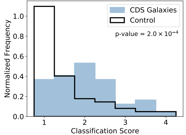
Figure 12. Distributions of merger classification scores for the CDS and control galaxy samples. A two-sample K-S test returns a p-value of \sim 2 \times 10^{-4} , confirming that these data are unlikely to come from the same parent distribution. The median score is 1.0 for the control galaxies compared to 2.0 for the CDS galaxies. Moreover, there are roughly twice as many "likely" mergers, i.e., galaxies with average score \geq 3.5 , in the CDS sample than in the control sample ( \sim 10\% versus \sim 5\% , respectively).
