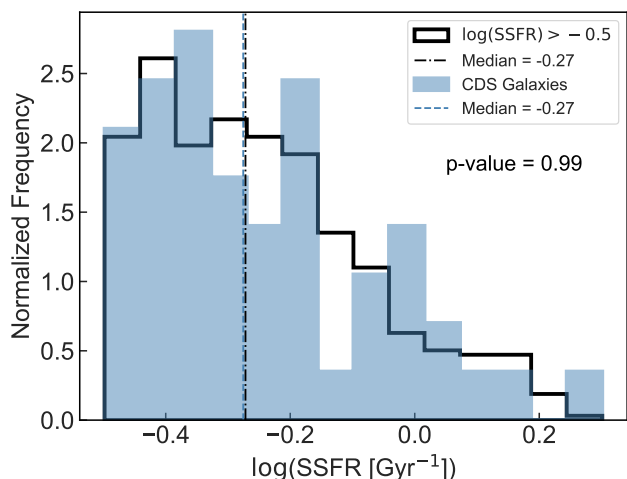
Figure 10. Distribution of RESOLVE galaxy SSFRs revealing that non-compact and compact star-forming galaxies follow same distribution of specific star formation rates at z \sim 0 . In contrast, Barro et al. (2013) find that high- z blue nuggets exhibit lower SSFRs than high- z non-compact star-forming galaxies (their Figure 4).
