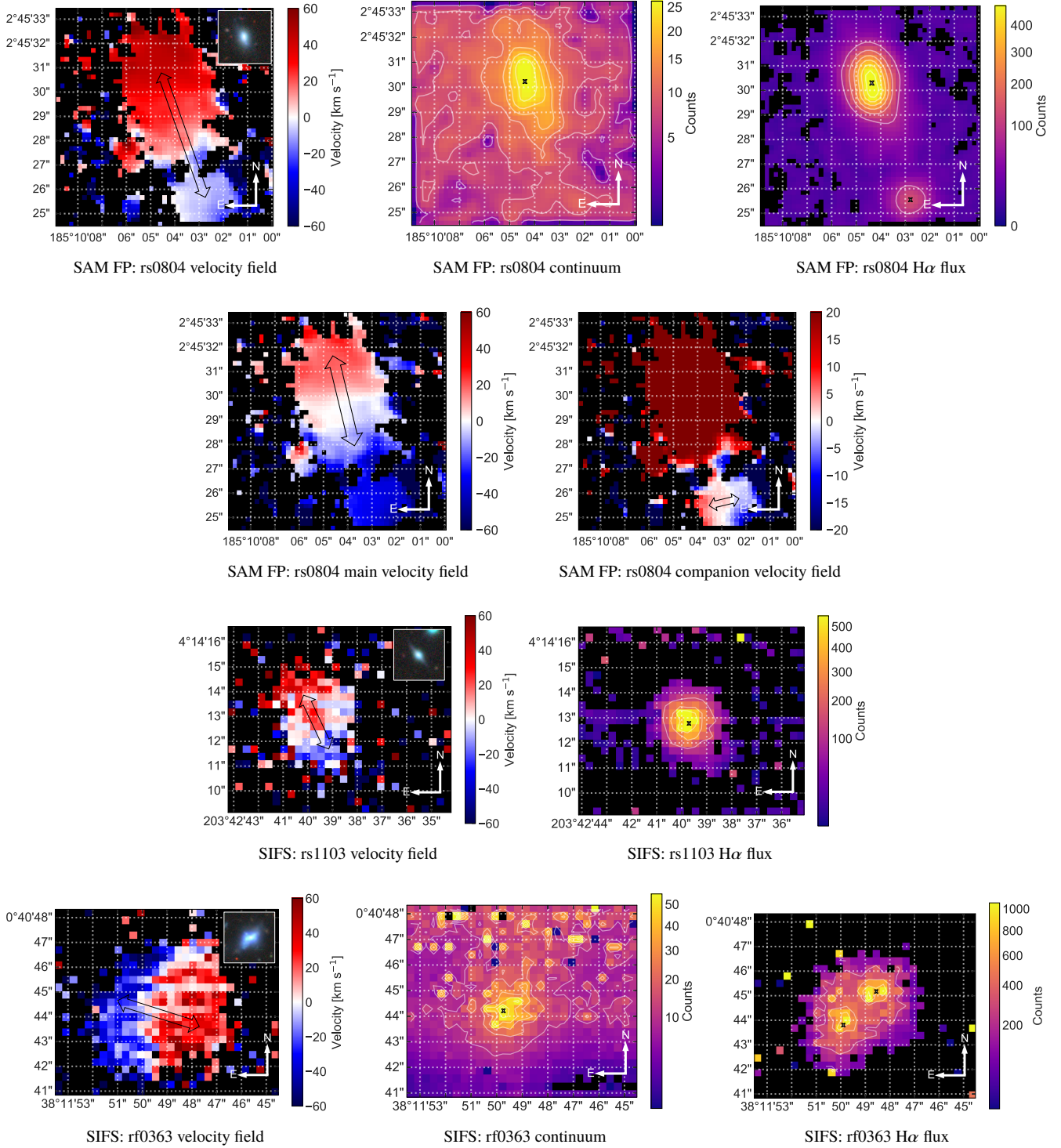
Figure 13. Same as previous page. Additional velocity fields are shown for the main object and the companion in the case of rs0804.
