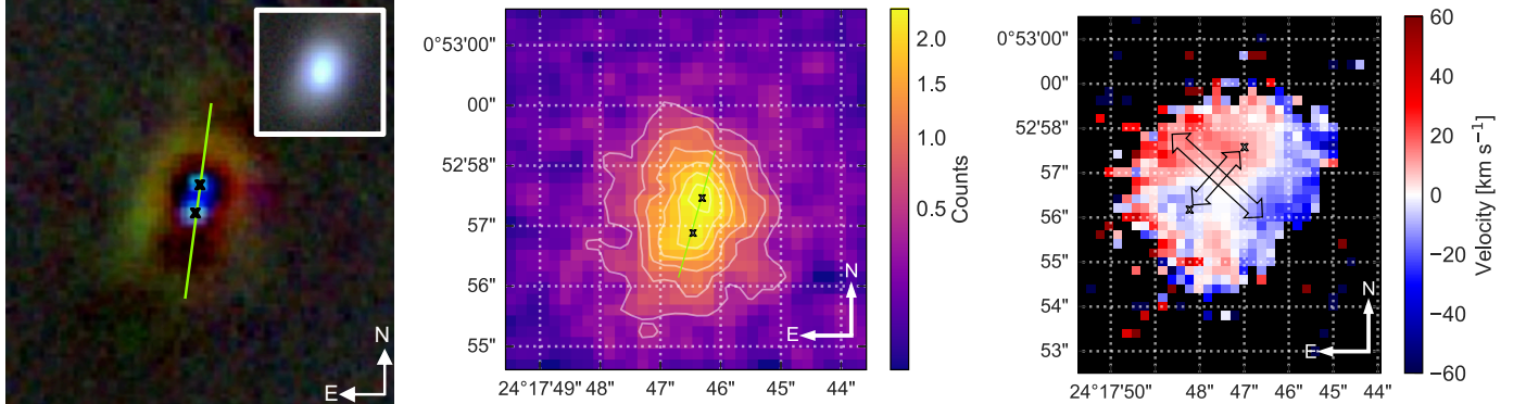
Figure 5. Merger confirmation in rf0250 by three methods. Left: Merger evidence, in the form of an apparent double nucleus, found by eye in DECaLS residuals. The green line corresponds to the approximate northeast alignment axis of the double nucleus. For reference, the DECaLS DR7 grz photometry is inset in the upper right corner. Middle: SAM FP continuum flux map for rf0250. Concentrations appear in two areas roughly matching the position of the apparent DECaLS nuclei. Right: GMOS IFU velocity field for rf0250. The inner velocity peaks (see §4.2.3) approximately align with the positions of the DECaLS double nucleus. Arrows in the right panel are drawn by eye to correspond to the numerically-identified positions of velocity maxima and minima, as described in §3.2. The mismatch between the absolute celestial coordinates of the GMOS and SAM FP images is the result of imprecisions in the GMOS IFU World Coordinate Solution as described in Appendix A.
