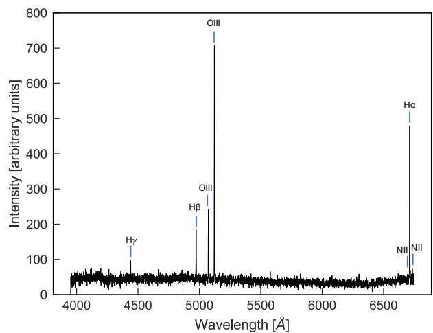
Figure 3. SOAR Integral Field Spectrograph (SIFS, see §2.3) spectrum for the RESOLVE CDS galaxy rs1103 displaying strong Balmer series and [OIII] emission lines typical of CDS galaxy spectra. The strong H\alpha emission signifies intense star formation, which is selected for by our UV- and IR-based SSFR restriction. The even stronger [OIII] emission lines relative to H\beta and [NII] are likely indicative of metal-poor gas (Pettini & Pagel 2004).
