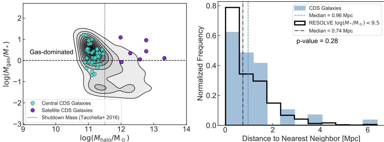
Figure 7. Left: CDS galaxies in RESOLVE generally occupy halos below the hot halo quenching threshold of M_{\text{halo}} \sim 10^{11.5} M_{\odot} and exhibit atomic gas-to-stellar mass ratios, M_{\text{gas}}/M_{*} , greater than unity. All but seven low- z CDS galaxies are the central galaxies (turquoise) in their halos; the rest are satellites (purple). The satellites are all highly gas rich, which may reflect recent infall into their groups or may indicate group-finding errors (see §2.1.1). Grayscale contours are drawn to correspond to the 10th, 20th, etc. percentiles of the probability density function. Right: Distribution of CDS nearest-neighbor distances revealing that they exist in environments similar to those of other dwarf galaxies, with if anything slightly larger nearest-neighbor distances.
