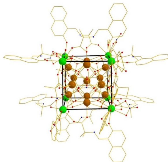
Figure 3. The crystal structure of 1 . Colour code: Ce III = green, Ce IV = brown, N = blue, O = red, C = gold. H-atoms omitted for clarity.
