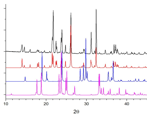
Fig.3. XRPD pattern of the Gly + Mal mixture following “dissolution” at 100% RH, and recrystallising under ambient atmosphere (ca 20% RH). The experimental XRPD (black) is shown alongside the simulated patterns for GSM (red), \alpha Gly (blue) and Mal (pink).
