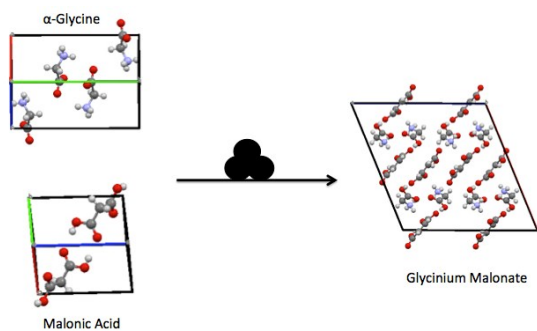
Fig. 1. Reaction scheme for the mechano-cocrystallisation of \alpha Gly + Mal to form glycinium malonate.
