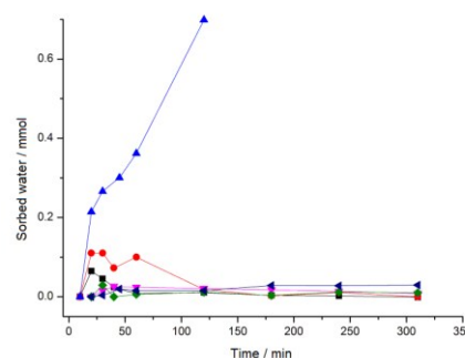
Fig.5. Water sorption of Gly + Mal mixture and GSM at various RH levels. \blacktriangle – Gly + Mal RH85%, \bullet – Gly + Mal RH 75%, \blacksquare – Gly + Mal RH65%, \blacktriangleleft , \blacktriangleright , \blacktriangledown – GSM at RH85%, 75%, 65%, respectively.
