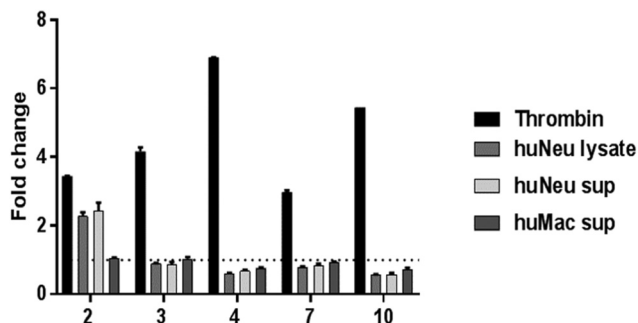
Fig. 3 Evaluation of the activation of FRET peptides 2, 3, 4, 7, 10 (10 μM) by Thrombin (5 U ml -1 ), human neutrophil (huNeu) lysates and supernatant (sup) and macrophage supernatant (huMac sup). Fold-changes in fluorescence (ex/em 485/528 nm) compared to probe in buffer only.
