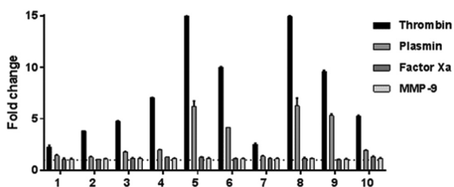
Fig. 2 Relative increase (fold change) in fluorescence of probes 1–10 (10 μM) after 10 min incubation with either Thrombin (5 U ml -1 ), Plasmin (30 nM), Factor Xa (0.5 μM) or MMP-9 (83 kDa, 30 nM), compared to control (probe in buffer alone (ex/em 485/528 nm)).
