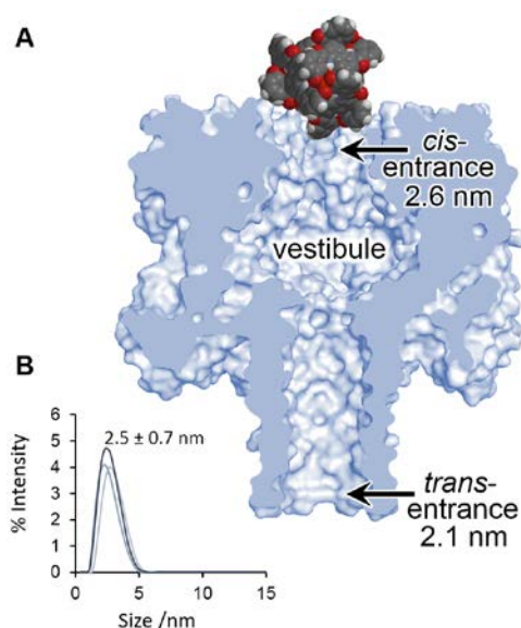
Figure 4. (A) Scaled model of a Ga(III) cage complex overlaid with the crystal structure of \alpha -HL. 44 (B) Dynamic light scattering measurement of a racemic sample of the Ga(III) cage complex in D_2O 293 \pm 2 K.
