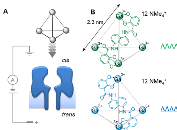
Figure 1. (A) Experimental setup in which tetrahedral coordination cages were driven towards the cis -opening of a single \alpha -haemolysin ( \alpha -HL) nanopore inserted in a lipid bilayer under an applied transmembrane potential. (B) \Lambda\Lambda\Lambda\Lambda (green) and \Delta\Delta\Delta\Delta (blue) homochiral forms of the Ga(III) cage used in this study. Each grey edge indicates the position of a bridging ligand molecule.
