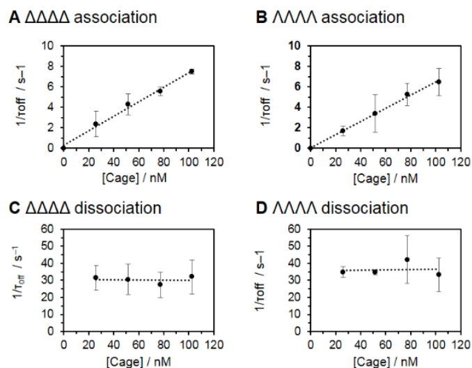
Figure 3. (A–D) Association and dissociation kinetics of the \Delta\Delta\Delta\Delta and \Lambda\Lambda\Lambda\Lambda cages with an \alpha -HL nanopore. The rate constant k_{on} was obtained from the slope of the linear fit of 1/\tau_{on} versus [cage] for \Delta\Delta\Delta\Delta (A) and \Lambda\Lambda\Lambda\Lambda (B). The rate constant k_{off} was obtained from the intercept of the graph 1/\tau_{off} versus [cage] for \Delta\Delta\Delta\Delta (C) and \Lambda\Lambda\Lambda\Lambda (D). Experiments were performed in 1 M KCl, 30 mM Tris-DCl, pH 7.6 in D_2O at 293 \pm 2 K with an applied potential of +100 mV.
