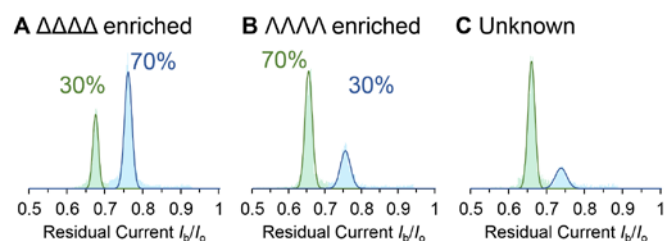
Figure 5. (A–C) Event distributions generated for enantio-enriched samples. Experiments were performed in 1 M KCl, 30 mM Tris-DCl, pD 7.6 in D 2 O at 293 ± 2 K with an applied potential of +100 mV.
