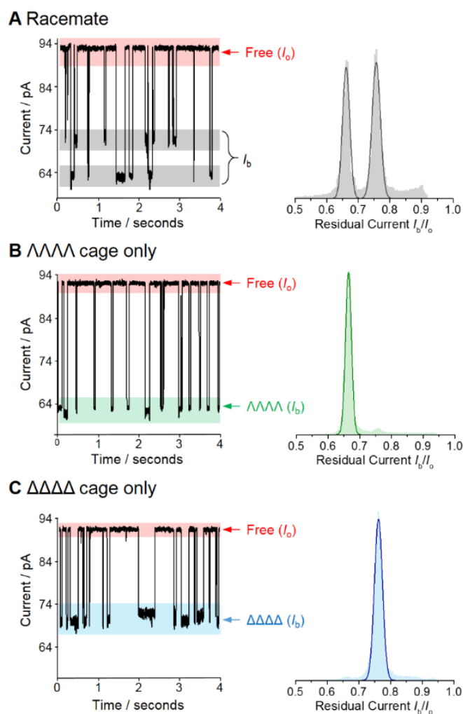
Figure 2. Enantiodiscrimination of Ga(III) coordination cages by an \alpha -HL nanopore at +100 mV. Representative ion current traces and corresponding event histograms for nanopore analysis of (A) a racemic mixture of the coordination cage, (B) enantiopure \Lambda\Lambda\Lambda cage, and (C) enantiopure \Delta\Delta\Delta cage. Each histogram was generated from at least six different experiments totaling >34,000 events in each case. Experiments were performed in 1 M KCl, 30 mM Tris-DCl, pD 7.6 in D 2 O at 293 \pm 2 K with an applied potential of +100 mV.
