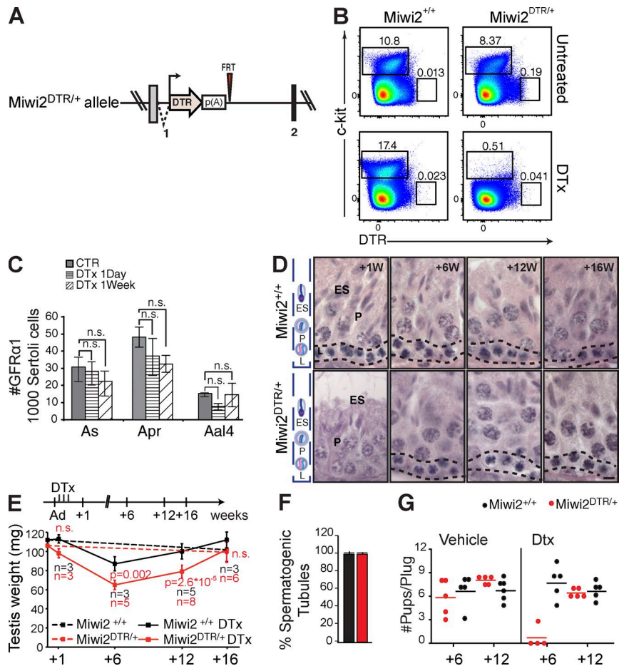
Figure 3. Miwi2-expressing cells are transit amplifying and do not contribute to the long-term maintenance of spermatogenesis. (A) Schematic overview of the Miwi2 DTR allele. (B) Representative FACS analysis of live CD45 Neg CD51 Neg gated cells is shown of testicular populations of wild-type and Miwi2 DTR/+ mice stained with c-kit and DTR antibodies (top) and after 3x DTx administrations analyzed 1 d after the last injection (bottom). Numbers indicate the percentages of cells of the defined subpopulations. (C) Enumeration of the GFRα1 Pos populations in adult Miwi2 +/+ mice that were untreated ( n = 3 ) or treated with 3x DTx injections and analyzed 1 d ( n = 4 ) or 1 wk (W; n = 4 ) after the last injection. Numbers represent cells of indicated chain length normalized to 1,000 sertoli cells. (D) Histology of testis; sections stained with H&E at time points indicated (1–16 wk [W]) after DTx administration are shown. Bar, 10 \mu m. (E) Testicular weight of the indicated cohorts at indicated time points. n, number of mice analyzed per time point. P-values are shown; n.s., no statistical significance. (F) Enumeration of fully spermatogenic tubules in wild-type and Miwi2 DTR/+ mice at the final 16 wk time point after DTx administration is shown. (G) Fertility as represented by pups per plug of the indicated cohorts at 6 and 12 wk after DTx or vehicle control injection. Black and red represent wild-type and Miwi2 DTR/+ Dtx-treated mice, respectively. Error bars represent SEM.
