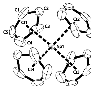
Figure 1. Thermal ellipsoid drawing (50 % probability for non-H atoms) of NpCp 4 in the solid state. H atoms omitted. Selected bond lengths [Å] and angles [°] for NpCp 4 : Np1-Ct 2.551(2), Np1-C 2.78(1) to 2.83(1), Ct-Np1-Ct 109.4(2).
