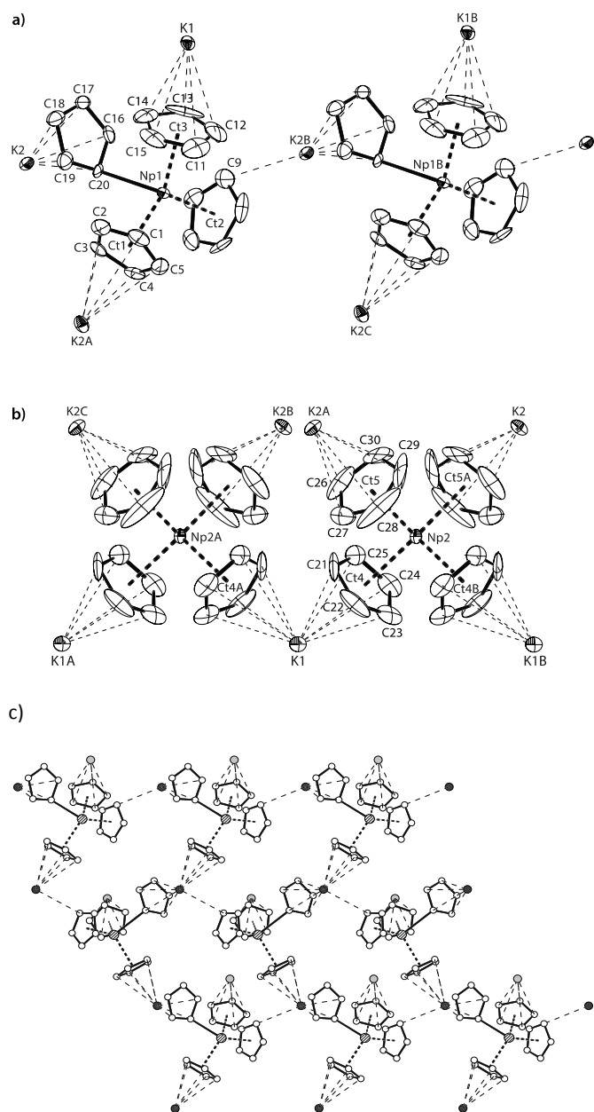
Figure 3. a) Thermal ellipsoid drawing of a portion of the polymeric structure type K[Np(\eta^5-Cp)_3(\eta^1-Cp)] formed by Np^{III} cations A, and b) the polymeric sheet-like structure type K[Np(\eta^5-Cp)_4] formed by Np^{III} cations B. Thermal ellipsoids for (a) and (b) are at 50% probability. c) Ball and stick drawing of part of the 2D-polymeric sheet structure formed by the type A Np^{III} cations and K2. Atom colours: C (white), K1 (light grey), K2 (dark grey), Np1 (filled with lines). Hydrogen atoms and lattice diethyl ether molecules are omitted for clarity. Symmetry generated atom names are labelled A, B and C. Selected distances [Å] and angles [°] for K[NpCp_4] : Np1-C20 2.752(7), Np1-Ct1 2.527(4), Np1-Ct2 2.516(4), Np1-Ct3 2.493(6), K1-Ct3 3.067(6), K1-Ct4 3.013(5), K2-C9 3.197(10), K2-C16 3.049(8), K2-C20 2.976(7), K2A-Ct1 3.003(5), K2-Ct5A 2.884(7), Ct1-Np1-Ct2 115.50(13), Ct1-Np1-Ct3 118.92(16), Ct2-Np1-Ct3 117.19(17), Np1-Np1-C20 96.53(16), Ct2-Np1-C20 99.01(17), Ct3-Np1-C20 103.51(19), Np2-Ct4 2.631(5), Np2-Ct5 2.645(7), Ct4-Np2-Ct5 109.2(2), Ct4-Np2-Ct4B 109.6(2), Ct4-Np2-Ct5A 110.5(2), Ct5-Np2-Ct5A 107.9(3), Ct4-K1-Ct4A 104.67(19), \phi(Ct4-Np2-Ct5\angle Ct4B-Np2-Ct5A) 88.7(2), \phi(Ct4-Np2-Ct4B\angle Ct5-Np2-Ct5A) 90.9(3).
