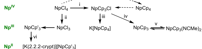
Scheme 1. Synthetic routes to neptunium complexes presented in this work. \text{NpCp}_3 is obtained by reduction from \text{NpCp}_3\text{Cl} and readily forms the MeCN stabilised solvate. The silylated analogue \text{Np}(\text{Cp}')_3 ( \text{Cp}' = \text{C}_5\text{H}_4\text{SiMe}_3 ) is better obtained from the reaction of \text{NpCl}_3 with \text{KCp}' and can be reduced to its K salt. Dotted lines indicate literature procedures. Key: (i) excess KCp, PhMe; (ii) Na/Hg, \text{Et}_2\text{O} , -NaCl; (iii) KCp, -KCl; (iv) Na/Hg, \text{Et}_2\text{O} , -NaCl; (v) excess MeCN; (vi) \text{KC}_8 , 2.2.2-cryptand, THF/ \text{Et}_2\text{O} , -8C.
