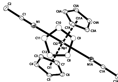
Figure 4. Thermal ellipsoid drawing (50% probability for non-H atoms) of NpCp_3(NCMe)_2 in the solid state. H atoms omitted. Selected bond lengths [Å] and angles [°] for NpCp_3(NCMe)_2 : Np1-N1 2.665(4), Np1-Ct1(a) 2.539(4), Np1-Ct2 2.540(4), N1-C1 1.135(5), C(1)-C(2) 1.465(5), N1-Np1-N1A 178.4(2), Ct-Np1-Ct: 116.9(2), 119.9(2), 123.5(2).
