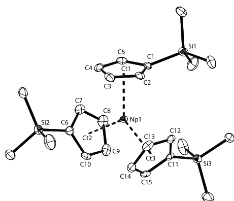
Figure 5. Thermal ellipsoid drawing (50 % probability for non-H atoms) of NpCp' 3 in the solid state. H atoms omitted. Selected bond lengths [Å] and angles [°]: Np1-Ct1 2.485(2), Np1-Ct2 2.481(2), Np1-Ct3 2.479(2), Np1-C ar 2.734(6) to 2.786(4), Si1-(C1-C5) plane -0.382(8), Si2-(C6-C10) plane -0.109(8), Si3-(C11-C15) plane -0.169(8), Ct1-Np1-Ct2 119.86(8), Ct1-Np1-Ct3 120.46(7), Ct2-Np1-Ct3 119.06(8).
