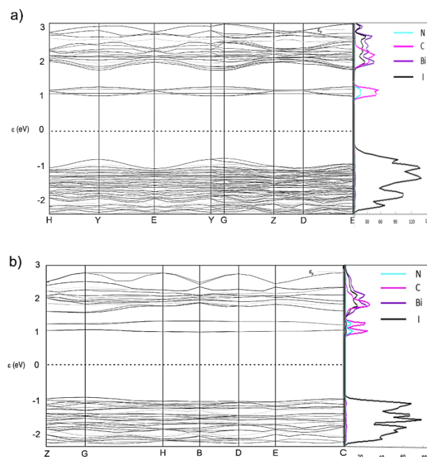
Figure 4. Band structures of [py][BiI 4 ] (a) and [mepy][BiI 4 ] (b), and corresponding projected DOS (6p orbital for bismuth: purple; 5p orbital for iodine: black; 2p orbital for nitrogen: cyan; 2p orbital for carbon: magenta). The Fermi level was set at 0 eV.
