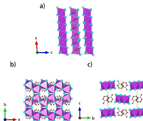
Figure 1. Crystallographic packing diagrams of [py][BiI 4 ] when viewed along different axes. Bismuth atoms and [BiI 6 ] 3− octahedra: magenta; iodine atoms: cyan; carbon atoms: brown; nitrogen atoms: violet. Hydrogen atoms are hidden for clarity.
