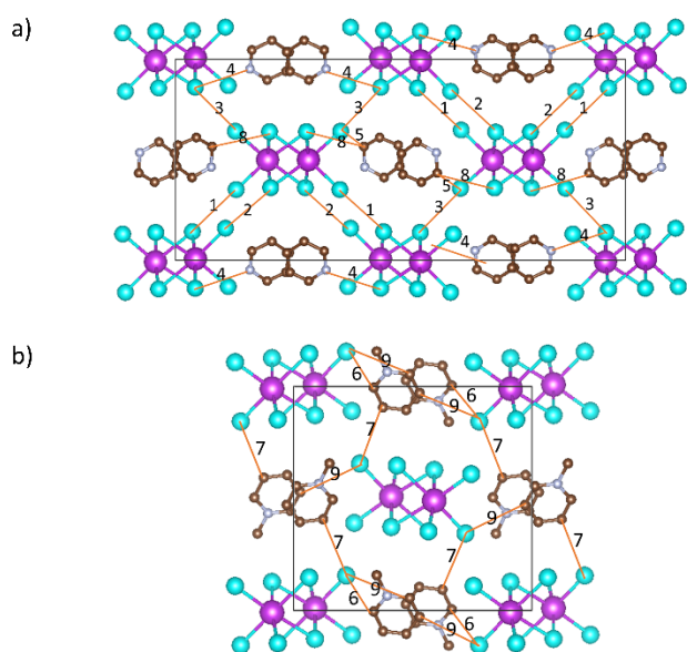
Figure 3. Intermolecular interactions (show in orange lines) in [py][BiI 4 ] (a) and [mepy][BiI 4 ] (b) unit cells. Image generated by VESTA (Visualization for Electronic and Structural Analysis) software. Bismuth atoms: magenta; iodine atoms: cyan; carbon atoms: brown; nitrogen atoms: violet. Hydrogen atoms are hidden for clarity.
