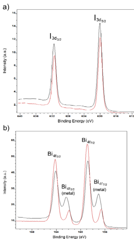
Figure 7. Iodine 3d (a) and bismuth 4f (b) XPS spectra for thin films of [py][BiI 4 ] (red) and [mepy][BiI 4 ] (black).
