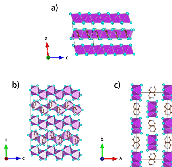
Figure 1. Crystallographic packing diagrams of [py][BiI 4 ] when viewed along different axes. Bismuth atoms and [BiI 6 ] 3− octahedra: magenta; iodine atoms: cyan; carbon atoms: brown; nitrogen atoms: violet. Hydrogen atoms are hidden for clarity.
