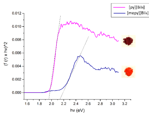
Figure 6. Tauc plots and bandgap estimations for [\text{py}][\text{BiI}_4] (magenta) and [\text{mepy}][\text{BiI}_4] (navy), powder samples diluted in \text{BaSO}_4 . Photos of both powders are shown on the right side to illustrate their appearance.
