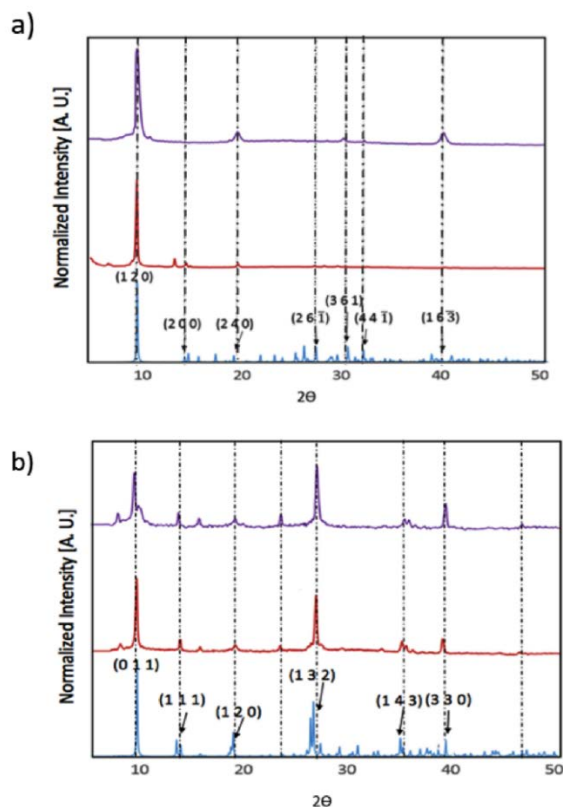
Figure 5. X-ray diffraction patterns for thin [\text{py}][\text{BiI}_4] film (top) and thin [\text{mepy}][\text{BiI}_4] film (bottom) on quartz glass slides, shown in normalized intensity versus 2\theta . Simulated pattern: blue; XRD pattern for thin-films: red; XRD pattern for thin-films after one-week exposure to the air in the dark: purple.
