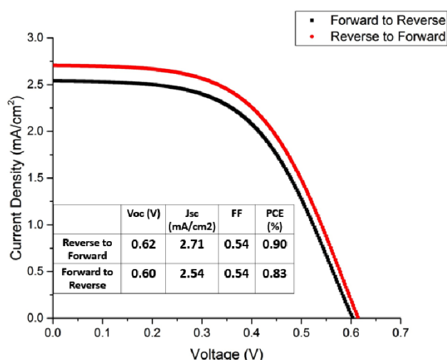
Figure 10. Boltzmann-fitted J-V curve of [py][BiI 4 ] champion cells.
