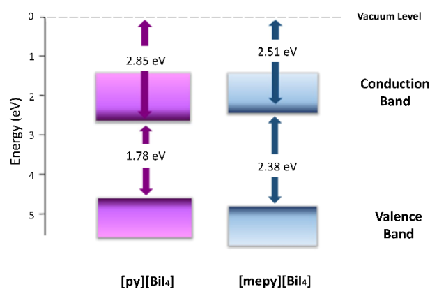
Figure 8. Energy level diagram for [py][BiI 4 ] and [mepy][BiI 4 ] , with E_{vac} set at 0 eV.
