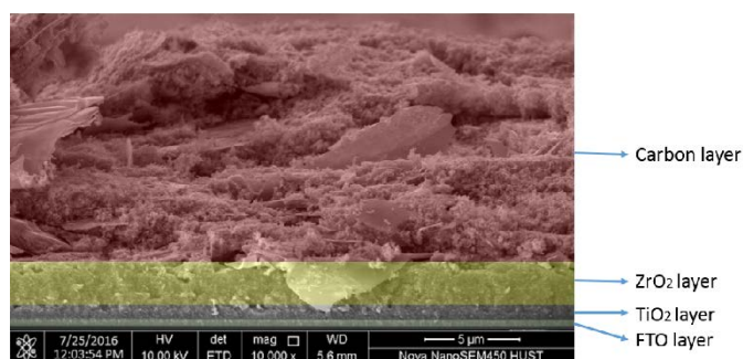
Figure 9. Cross-sectional SEM image of the mesoscopic triple-layer solar cell architecture.
