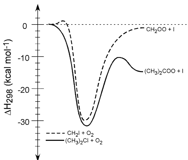
Figure 2. Calculated enthalpies for the stationary points in reactions of CH_2I and (CH_3)_2CI radicals with O_2 to form I atom and the corresponding Criegee intermediates, shown relative to the initial reactants at zero.
