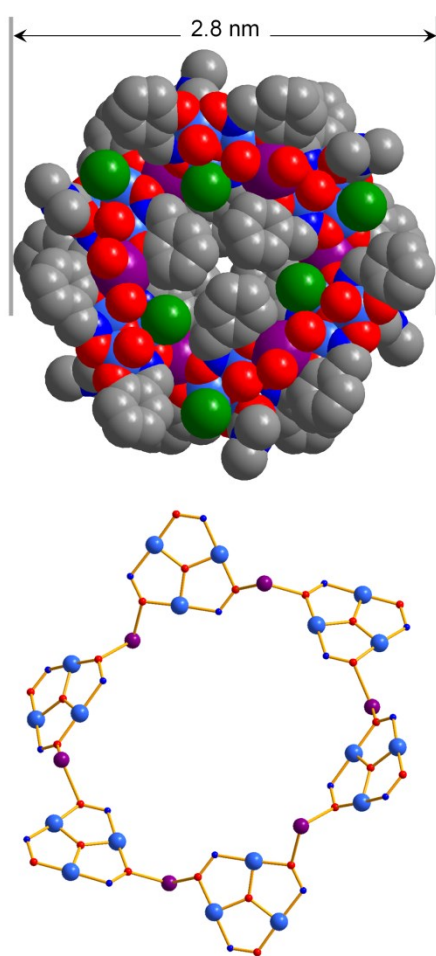
Fig. 2 Space-filling representation of the molecular structure of 1 , emphasizing its nano-sized dimensions (top). The structural core of 1 highlighting the [Mn 3 ] triangles linked through Na + ions (bottom). Colour code: Mn blue; Na, purple; Br, green; O, red; N, dark blue; C, grey. H atoms are omitted for clarity.
