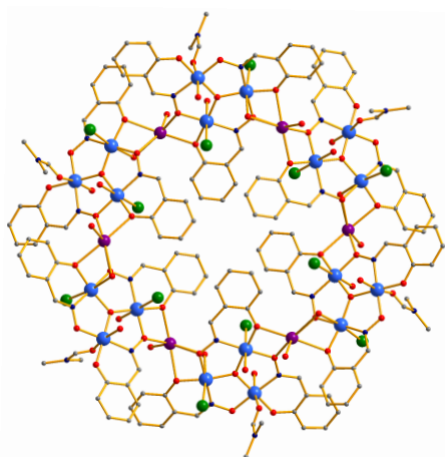
Fig. 1 Representation of the molecular structure of 1 . Colour code: Mn blue; Na, purple; Br, green; O, red; N, dark blue; C, grey. H atoms are omitted for clarity.
