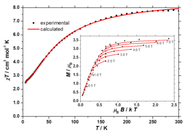
Fig. 3 \chi T product of 1 versus T plotted per [\text{Mn}^{\text{III}}_3] triangle. Insert: Variable temperature-and-variable-field (VTVB) magnetisation data of 1 in the field range 0.5 to 7.0 \text{ T} and in the temperature range 2 to 7 \text{ K} . The experimental data are shown as black circles. The calculated curves, obtained from full matrix diagonalization of spin-Hamiltonian (1) for isolated \text{Mn}^{\text{III}}_3 triangles, are shown as solid red lines.
