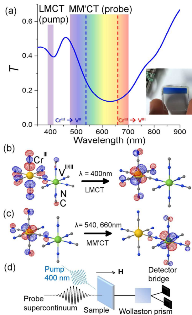
Figure 1: Orbital configuration and transmission associated to the ligand-to-metal and metal-to-metal charge transfer. (a) Static optical transmission spectrum of the film at room temperature. The pump wavelength is assigned to the ligand-to-metal charge transfer (LMCT) transition. The probe wavelengths span the visible part of the spectrum and measure changes related to the metal-to-metal charge-transfer (MM'CT) transitions for the two different V oxidation states present in the material. A photo of the film is shown in the inset. TD-DFT computations show (b) the LMCT transition and (c) the MM'CT transition. (d) Sketch of the femtosecond MO Faraday experimental setup.
