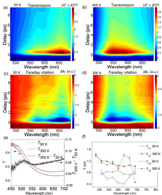
Figure 3: Spectro-temporal dynamics of the transmission and magneto-optical Faraday response for T_K = 50 and 300 K. (a) – (b) \Delta T/T and (c) – (d) \Delta\theta_F as a function of wavelength and time delay. (e) Static transmission spectra as a function of temperature. (f) Fitted time constants from the data in (a) – (d).
