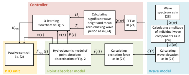
Fig. 6. Workflow diagram of the program used to simulate the point absorber.
