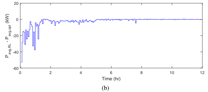
Fig. 10. RL-control-selected and optimal PTO damping coefficient (a) and difference in the corresponding mean absorbed power (b) in irregular waves with H_s = 2 m and T_z = 7 m, generated using a JONSWAP spectrum.
