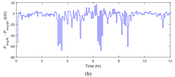
Fig. 12. Optimal and RL-control-selected ( J = 1, K = 4, L = 5 ) PTO damping coefficient (a) and corresponding mean absorbed power (b) in irregular waves with four sea states, generated from the combination of H_s = 2, 3 m and T_z = 7, 8 s.
