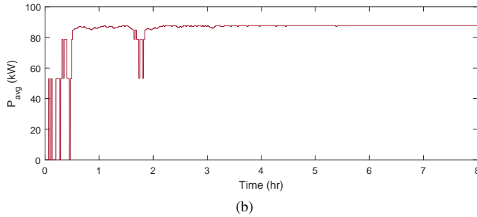
Fig. 8. RL-control-selected PTO damping coefficient (a) and corresponding mean generated power (b) in regular waves with H_s = 2.2 m and T_z = 8 s, when F_{Max} = 237.910 kN.
