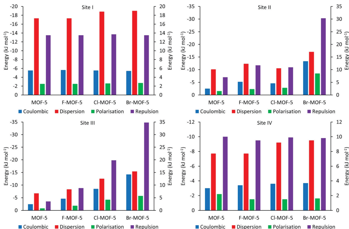
Fig. 10 PIXEL component energies for the four H 2 adsorption sites in MOF-5 and its halogen functionalised analogues. Repulsion bars correspond to the right hand axis, others to the left axis.
