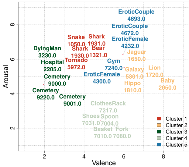
Fig. 8 Selection of the five most likely IAPS cases per cluster, for the k = 5 clustering solution, along with IAPS image codes. The color coding was chosen to be consistent with Fig. 7 above
