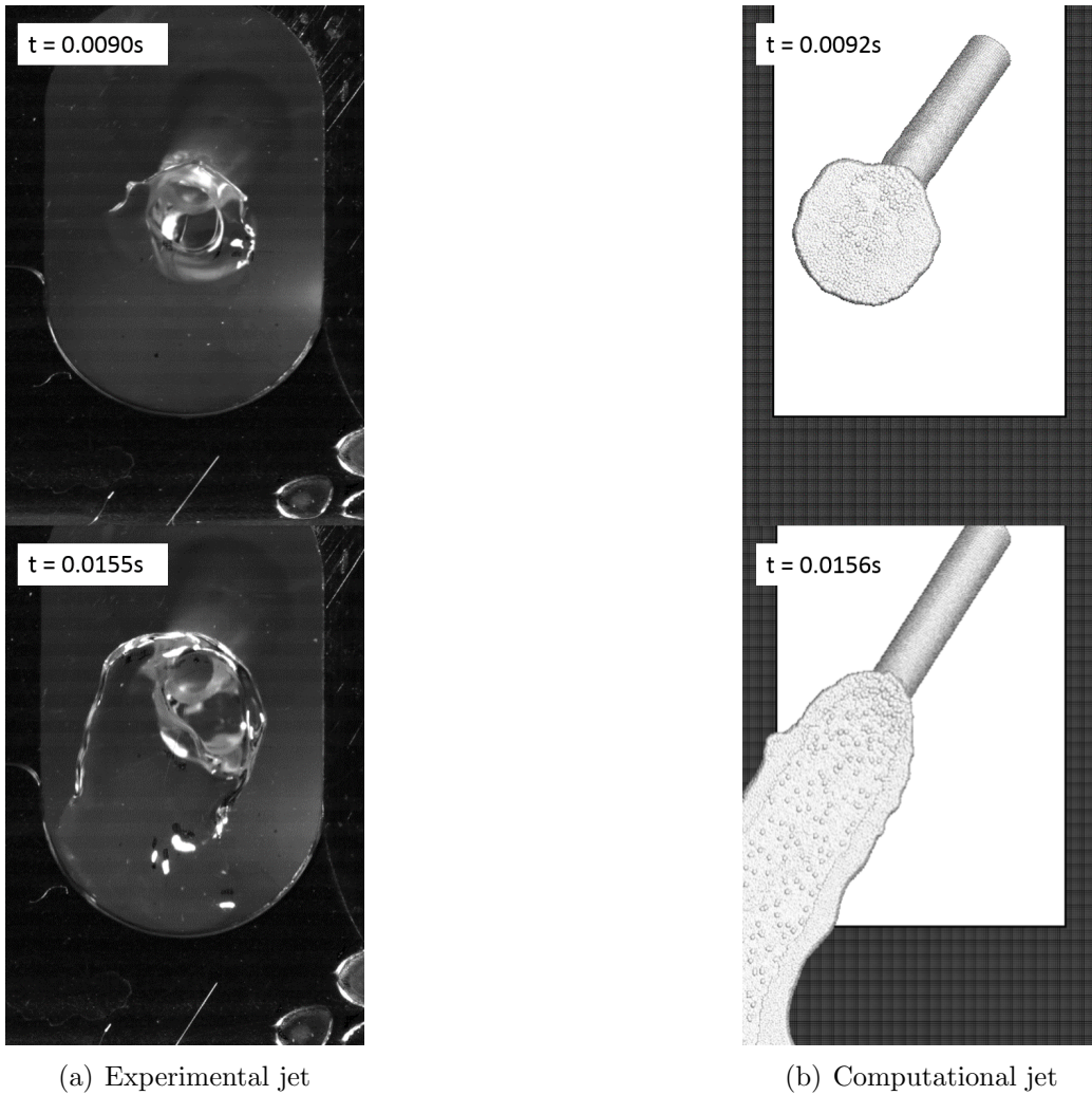
Figure 8: Shape formed by jet impinging on the plate
