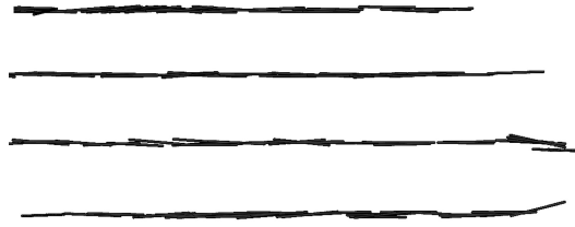
Figure 13: Fibre alignment for plate spacings of 0.3 mm for jet velocities of 0.4 m/s, 0.8 m/s, 1.6 m/s, 3.2 m/s (top to bottom)
