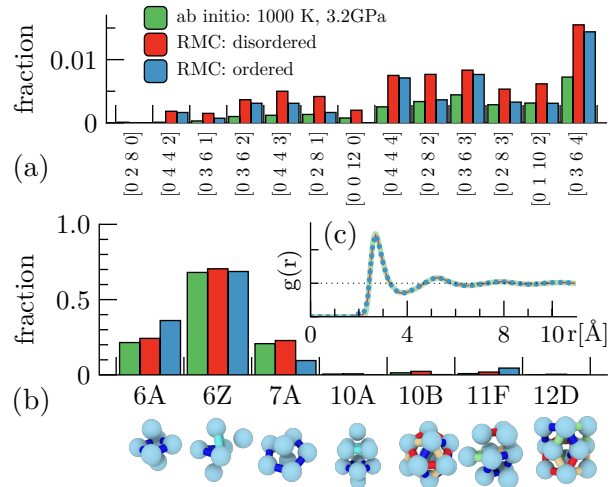
FIG. 4. Comparison of structural features between ab initio MD and RMC for a selected state point and two distinct seeds for the RMC fitting: an ordered and a disordered configuration. (a) Voronoi spectrum. (b) TCC spectrum. The structural motifs are illustrated with rings indicated by colored bonds. (c) Pair distribution functions from ab initio MD (green background) and the two RMC fits (overlapping blue dots and red line).
