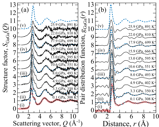
FIG. 2. (a) Structure factors S_{\text{GaGa}}(Q) measured in the DAC by SXR, and (b) corresponding pair distribution functions g_{\text{GaGa}}(r) obtained by Fourier transformation (black curves). Previously reported ambient- p measurements [63] are represented by the open red circles. A selection of the S_{\text{GaGa}} and g_{\text{GaGa}}(r) functions computed from the ab initio MD trajectories are also shown at comparable conditions just above the melting curve at (i) 303 K, (ii) 3.4 GPa, 400 K, (iii) 10.9 GPa, 600 K, (iv) 18.3 GPa, 800 K, and (v) 33.4 GPa, 1000 K (dashed blue curves).
