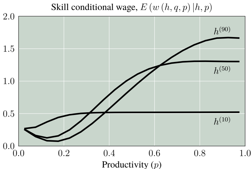
Figure 1: Non-monotone wages
