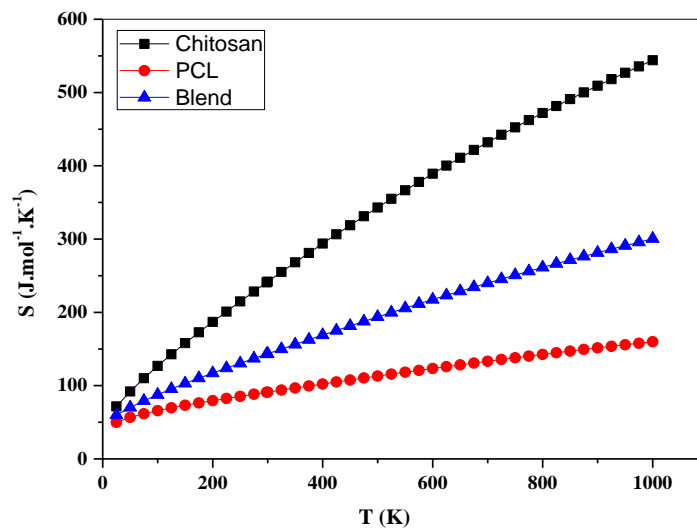
Figure (2) temperature versus entropy of the studied samples
