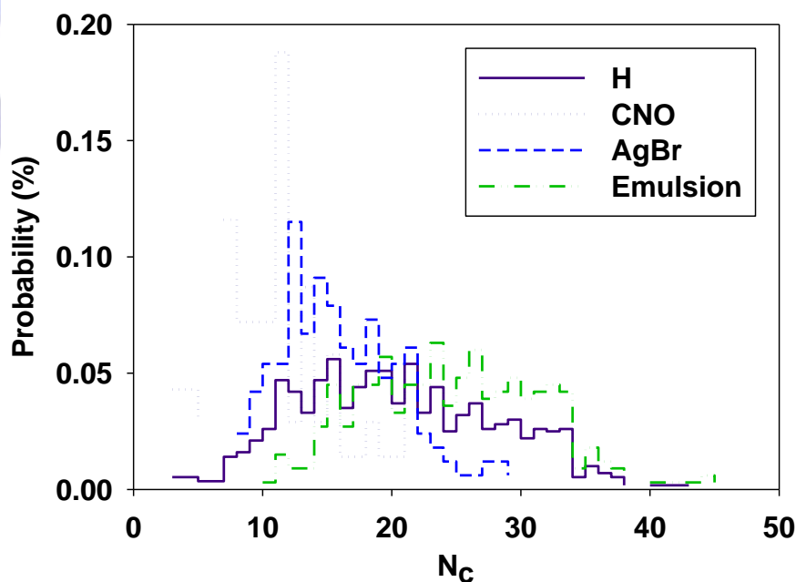
Fig 1: Compound multiplicity distribution for different emulsion targets in pion-nucleus interactions.
