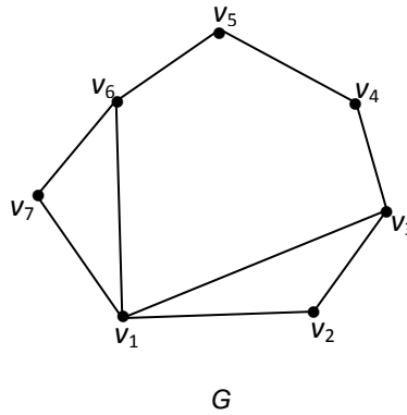
Figure 10 A graph G with rad G = 2 , diam G = 3 and om_l(G) = 3 .
