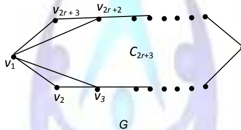
Figure 11 A graph G with rad G = r , diam G = r + 1 and om_l(G) = 3 .
