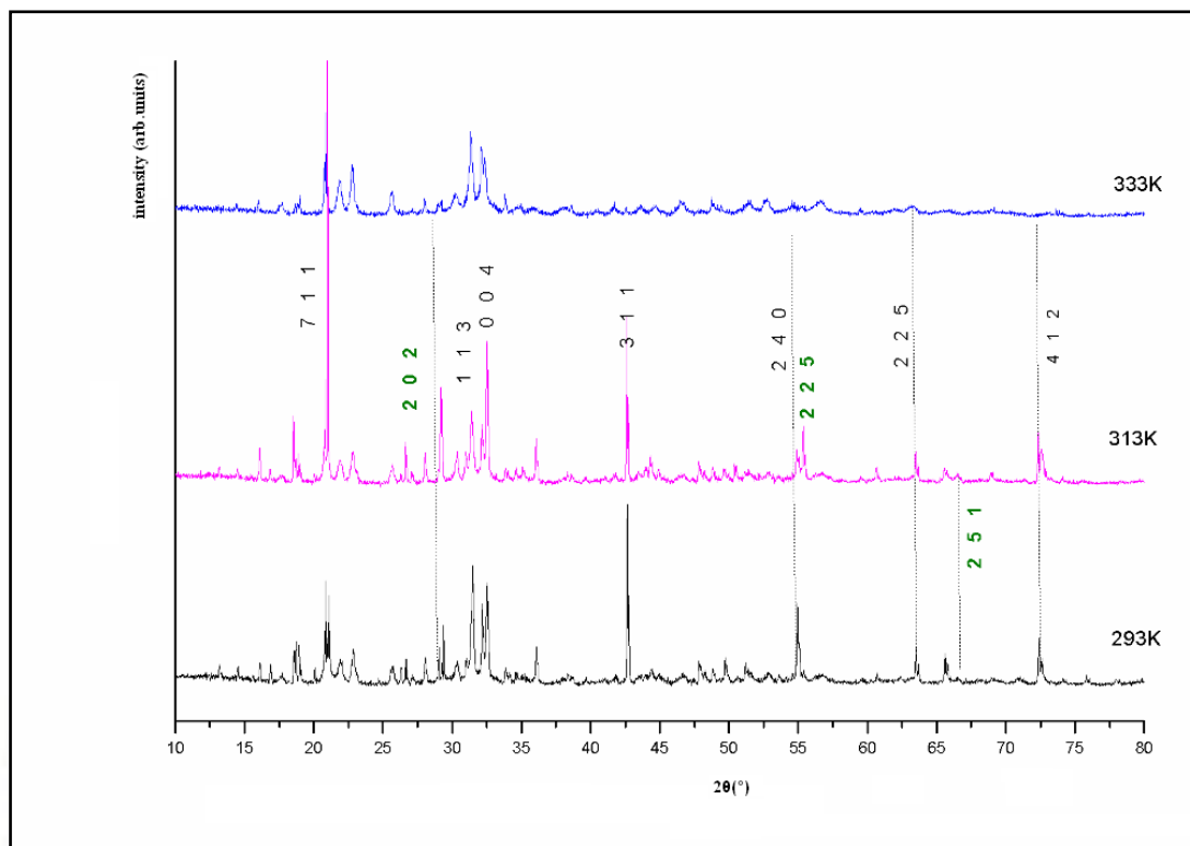
Fig.2. X-ray powder diffraction for NDAP material at 293; 313 and 333 K
