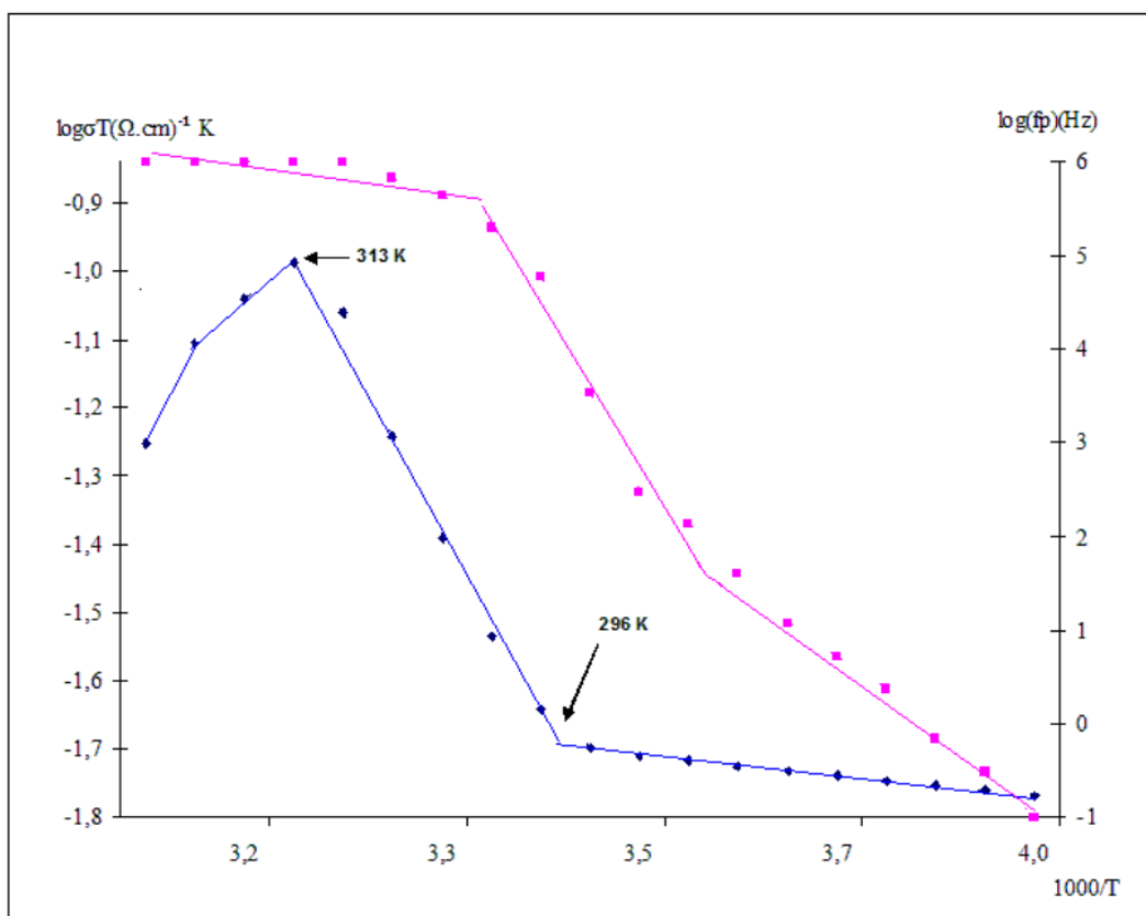
Fig.3. Temperature dependencies of \log(\sigma T) and \log fp = f(1000/T) , where fp is the M + max peak frequency for NDAP
