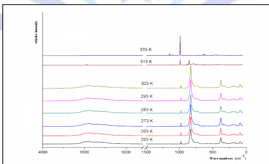
Fig.1. Raman spectra of crystalline \text{NaH}_2(\text{PO}_4)_{0.48}(\text{AsO}_4)_{0.52}\cdot\text{H}_2\text{O} between 253 and 333 K
