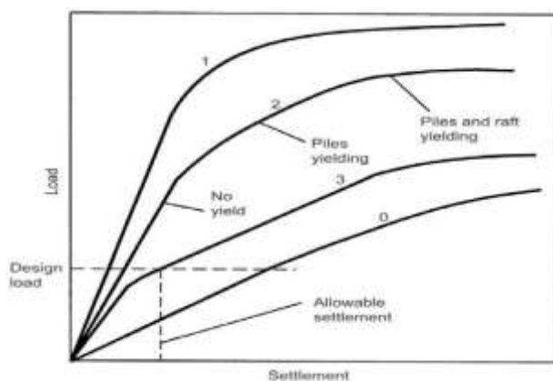
Figure 2 Load-settlement curves (Poulos, 2001)
