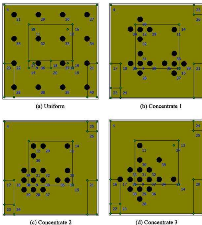
Figure 6 Different types of pile arrangement (Nguyen et al., 2014)
