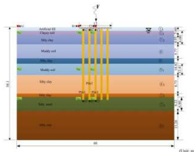
Figure 1 Piled raft foundation and details of geographic profile (Gu, Ye, Bao, & Zhang, 2016).
