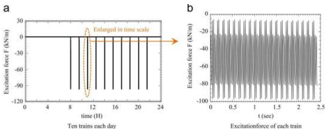
Figure 5 Loading due to high-speed train in one day (Gu, Ye, Bao, & Zhang, 2016).
