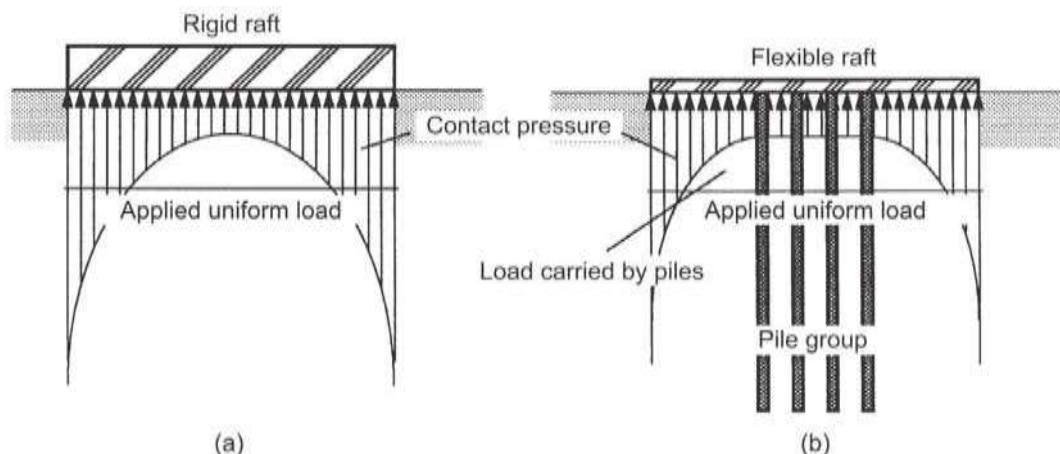
Figure 4 Distribution of contact pressure (a) rigid and (b) flexible rafts (Horikoshi & Randolph, 1998)
