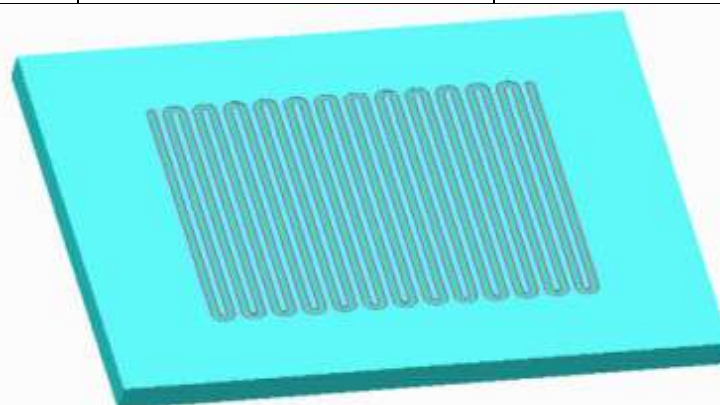
Fig. 1: Model of serpentine channel flow field of PEM fuel cell
