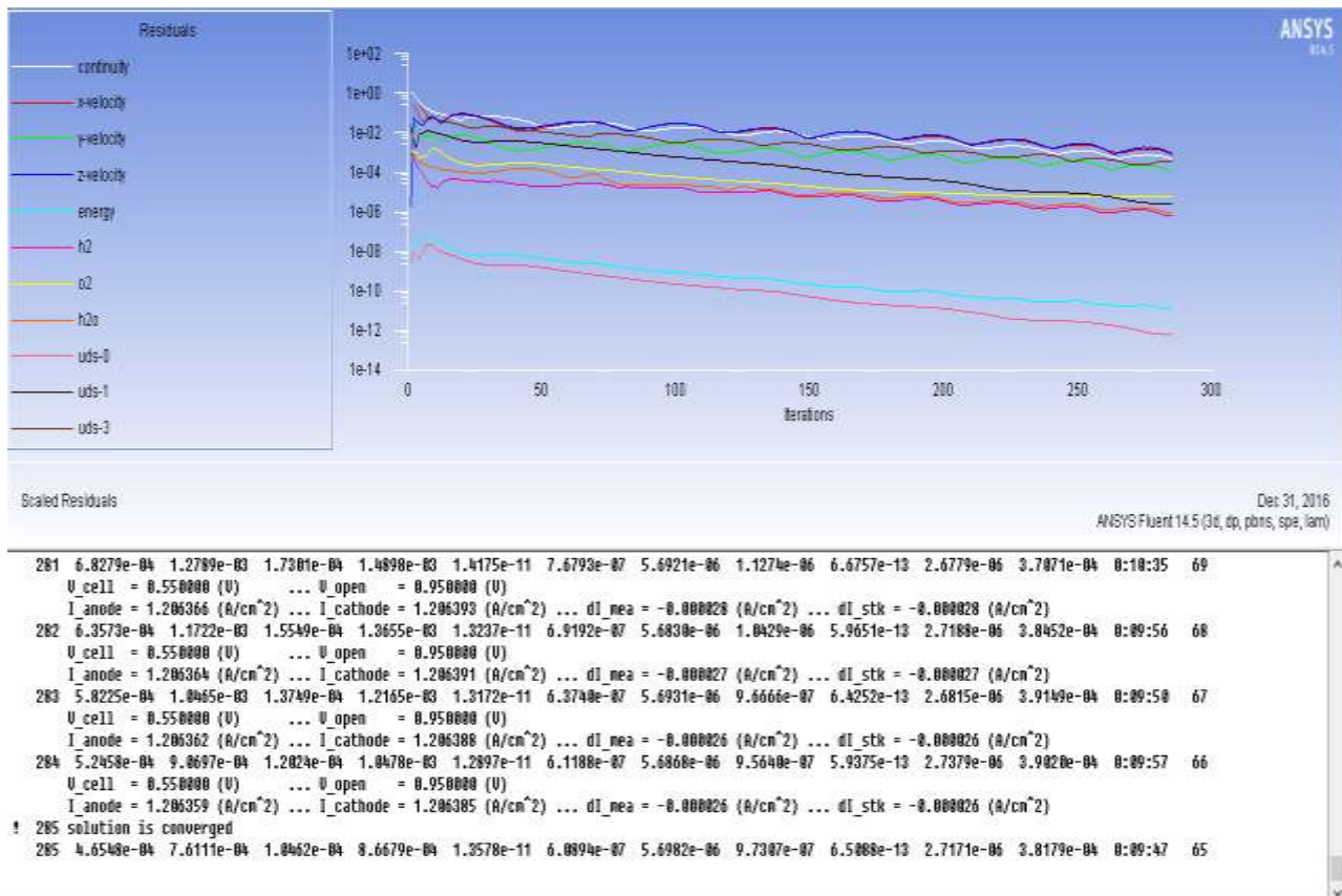
Fig. 5: Result for pressure of 1 bar at 0.55V
