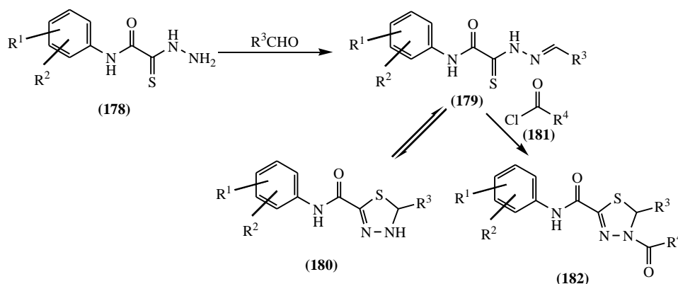
Scheme 44
