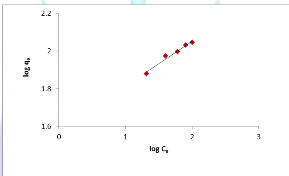
Fig 8: Freundlich isotherm plot of the adsorption of eosin dye onto activated carbon.
