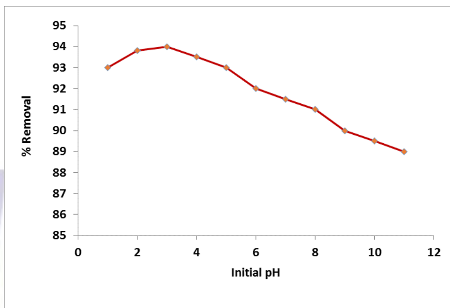
Fig 6: Effect of pH on removal of eosin dye by the prepared activated carbon from palm trunks, adsorbent dose (0.6 g) agitation time 50 min; 50 mL of eosin dye ( 10 \text{ mgL}^{-1} ).
