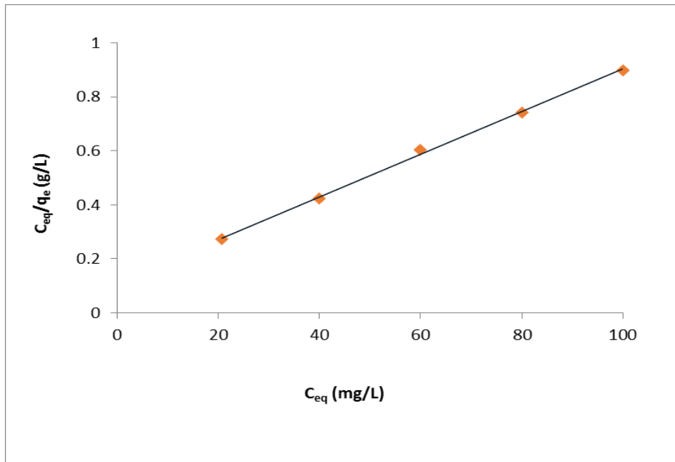
Fig 7: Plot of Langmuir adsorption isotherm of eosin dye onto powdered activated carbon.
