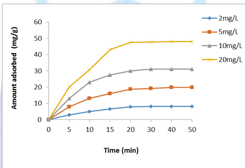
Fig 3: The variation of adsorption capacity with contact time at various initial dye concentration at 25\text{ }^{\circ}\text{C} (adsorbent= 0.2 g, V= 50 mL).
