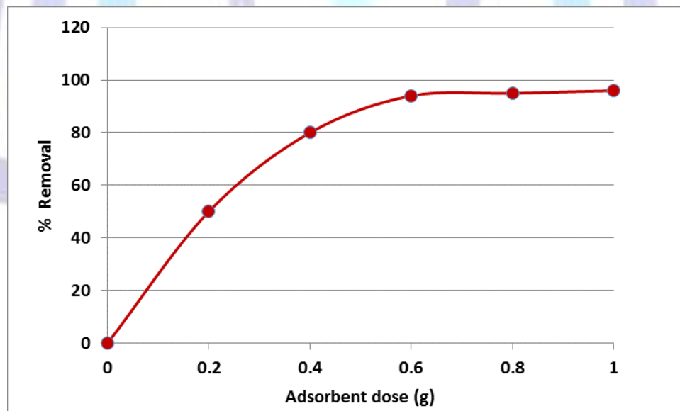
Fig 5: Effect of adsorbent dosage on removal of eosin dye; agitation time (50 min), 50 mL of eosin dye ( 10 \text{ mg L}^{-1} ).
