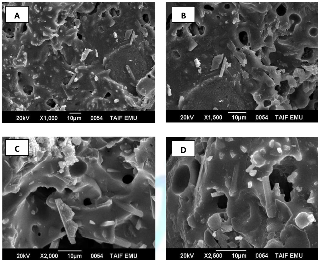
Fig 4: SEM micrographs of the fabricated activated carbon after adsorption of eosin dye molecules using different magnifications: (A) 1000 ×, (B) 1500 ×, (C) 2000 ×, and (D) 2500 ×.
