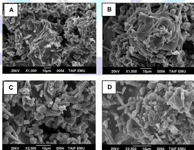
Fig 2: SEM micrographs of the fabricated activated carbon using different magnifications: (A) 1000 ×, (B) 1500 ×, (C) 2000 ×, and (D) 2500 ×.
