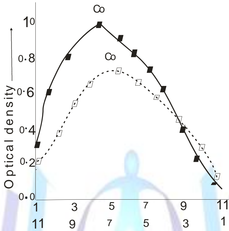
COMPOSITION OF THE Co(II)- CDHBOX COMPLEX BY JOB'S METHOD.
