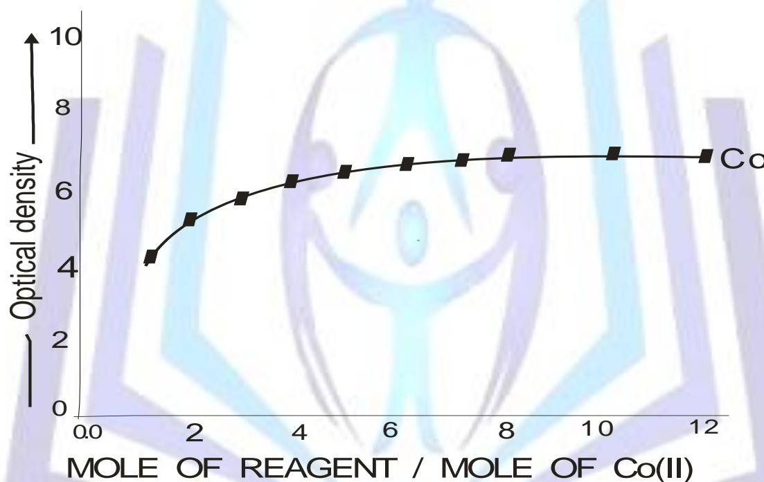
COMPOSITION OF THE Co(II)- CDHBOX COMPLEX BY MOLE RATIO METHOD
