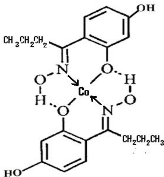
Proposed structure of Co(II)-HMAOX complex
