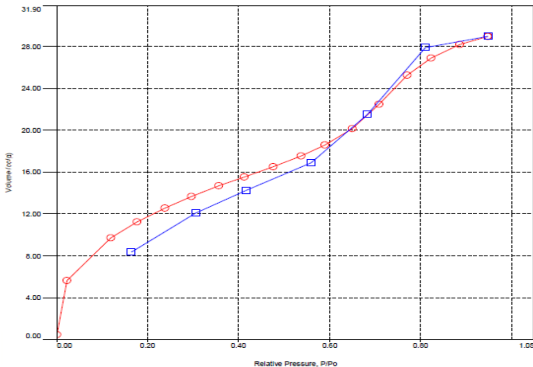
Figure 5: Adsorption-desorption isotherm of nitrogen onto S47 prepared sample.
