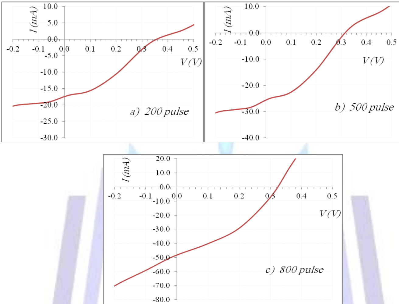
Figure (2): I-V characteristics of SSDSSC with \text{TiO}_2 at different No. of Nd:YAG laser pulses { (a-200), (b-500), (c-800) and CuI hole transport material kept at constant No. of pulse (800pulse) }.
