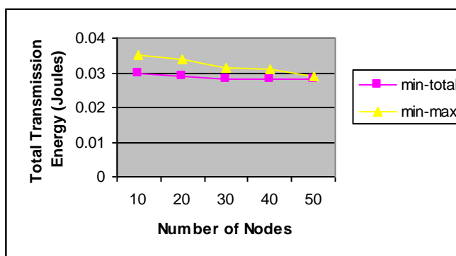
Figure 5. Total transmission energy by varying nodes
