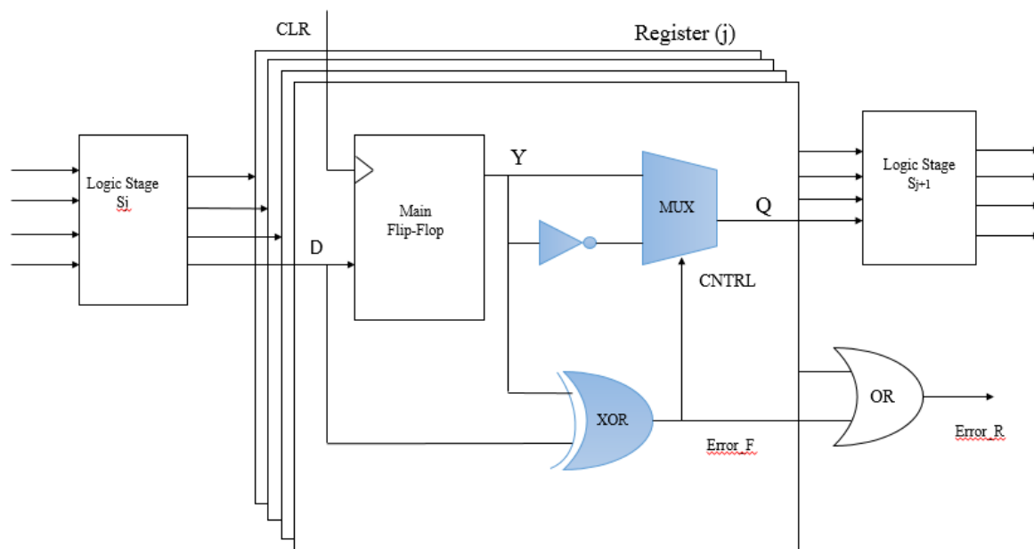
Figure 1:Proposed Circuit
