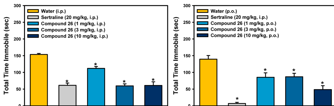
Figure 2. Mouse forced swim data for compound 26. The selective serotonin reuptake inhibitor, sertraline, produced the expected decrease in immobility. ANOVAs: F(4,43) = 34.20, p < 0.001 (left); F(4,44) = 20.75, p < 0.001 (right). *Fisher's PLSD posthoc test: p_s < 0.05 vs vehicle. n = 9-10 /group.
