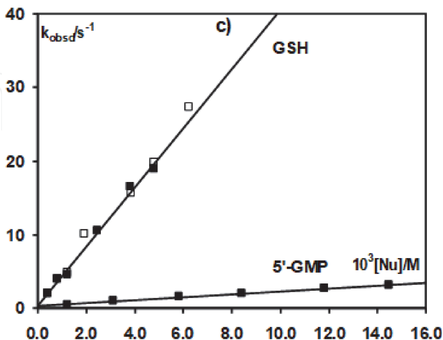
Figure 2. Observed pseudo-first-order rate constants, k_{\text{obsd}} as a function of nucleophile concentration at 37°C for 5'-GMP and GSH without 5'-GMP (open square) and in the presence of excess of 5'-GMP (full square) [7].
