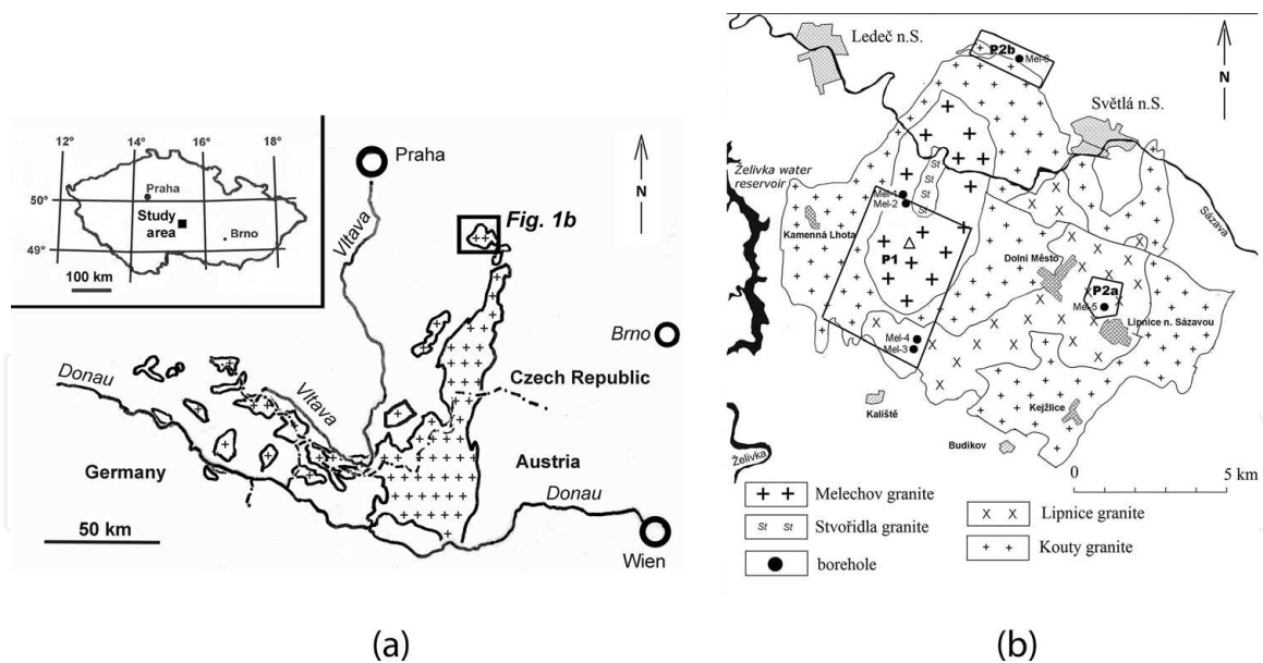
Figure 1. (a) Situation of the Melechov Massif in the Czech Republic and in the Moldanubian Batholith (delimitation of the batholith from Misař et al. [15]). (b) Granites of the Melechov Massif [10] with localization of boreholes and polygons of geochemical mapping. Triangle indicates the top of Melechov (715 m).
