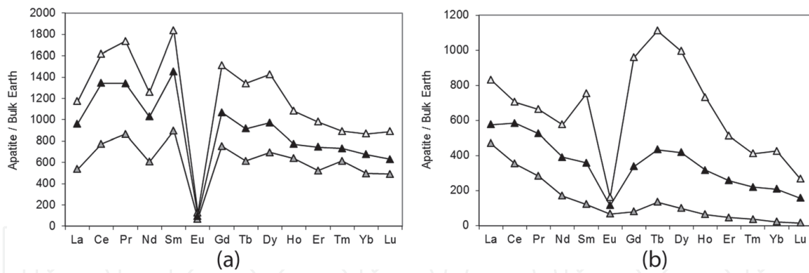
Figure 7. Bulk Earth normalized [51] REE in apatite (minimum, maximum, and median) as determined by LA-ICP-MS in polished sections of rocks: (a) Lipnice granite, Dolní Město—Kopaniny. (b) Melechov granite, Leštinka.
