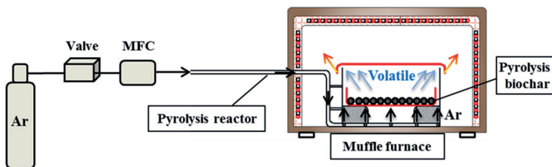
Figure 1. Biochar catalyst preparation using a muffle furnace.
