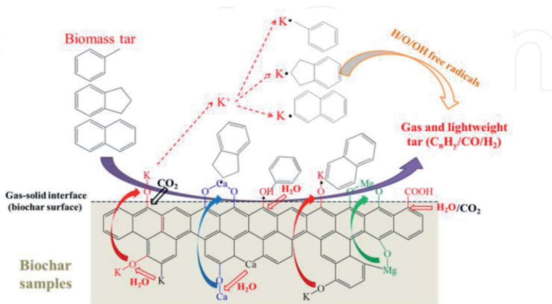
Figure 12. Heterogeneous reforming mechanism of biomass tar over biochar in the presence of \text{H}_2\text{O} and \text{CO}_2 at 800^\circ\text{C} [52].
