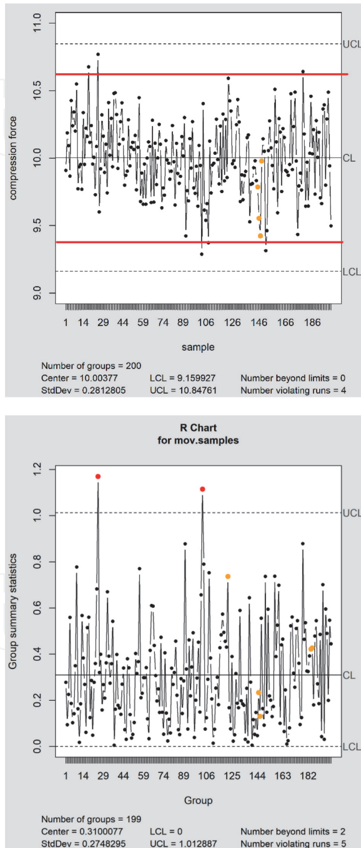
Figure 2. Control charts for compaction process: (upper) x-bar control chart and (lower) MR-chart (UCL = upper control limit; LCL = lower control limit; CL = mean or average range for the MR-chart). The red line corresponds to the warning limits using a RSD of 6%.
