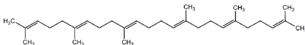
Figure 1. Structure of squalene.
