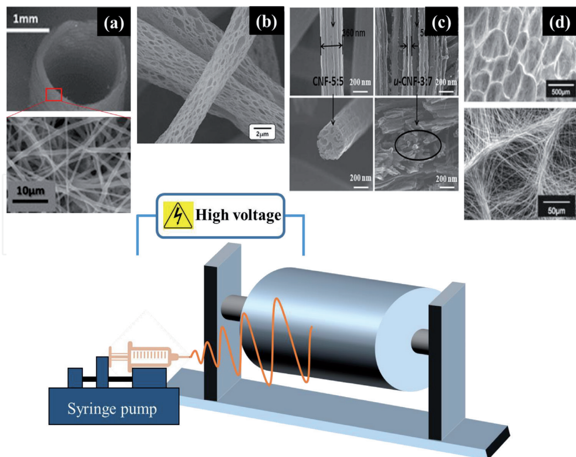
Figure 2. Electrospinning technique to fabricate nanofibers with different morphology (a) poly( \epsilon -caprolactone)-poly( l -lactic acid) nanofiber tubes [10], (b) cellulose acetate nanofibers with morphology control [11], (c) porous carbon nanofibers [12], and (d) cellulose acetate nanofibers with honeycomb-like surface structure [13].
