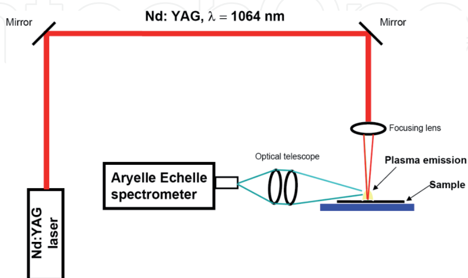
Figure 1. Layout of LIBS experimental setup.
