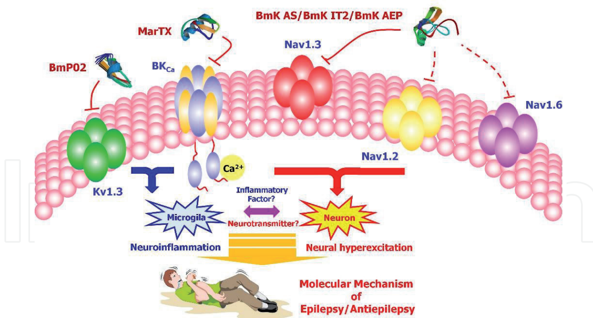
Figure 4. Antiepilepsy effects of BmK venom toxins by targeting Na + /K + channels. Long-chain \beta toxins BmK IT 2 /BmK AS/BmK AEP could reduce the epileptic seizure by inhibiting the activities of VGSCs. The specific BK channel blocker MarTX, a short-chain BmK toxin, suppressed the epilepsy by acting on the fAHPs and rapid spike repolarization of neurons, which might affect the activation of microglia through BK channels. BmP0 2 , a Kv1.3 inhibitor, has potential antiepileptic effects also by regulating the activation of microglia.
