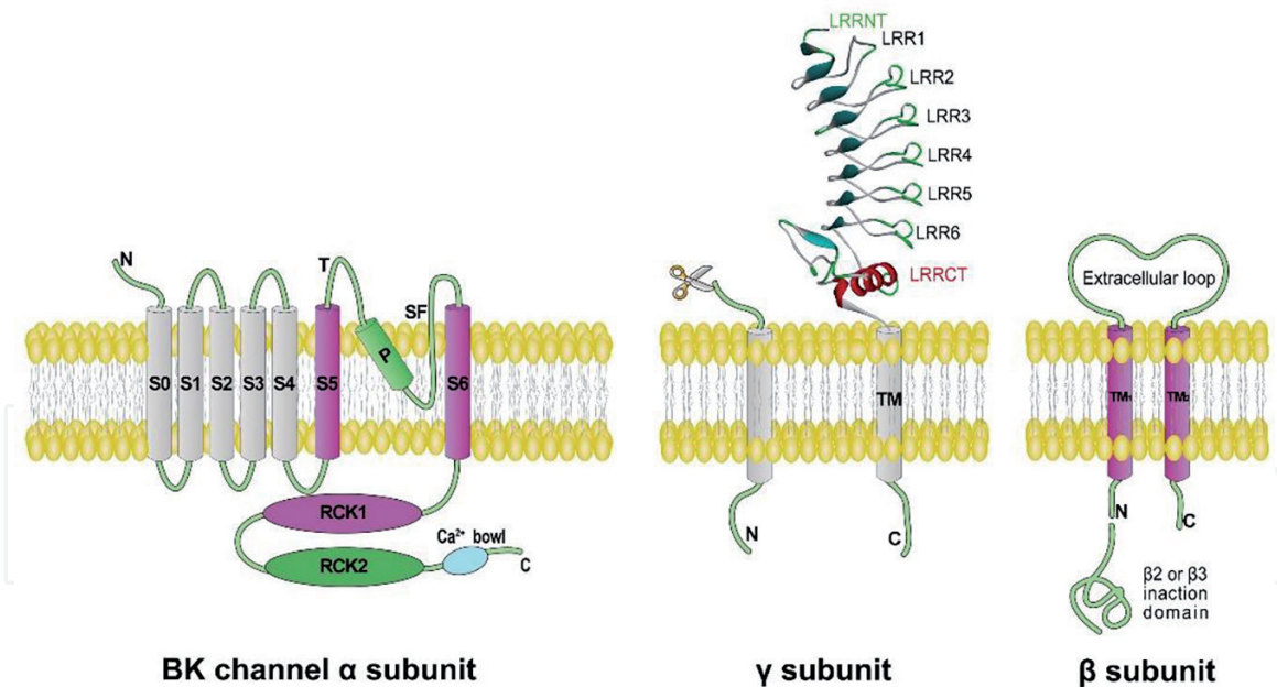
Figure 3. Structure of BK channel and its auxiliary subunits. BK channel topology predicted by the hydrophilicity profiles (left). The \alpha helices are represented by a cylindrical shape and S0 to S4 segments (gray column) make up the voltage sensor domain. The turret (T) is the loop joining S5 with the pore helix (P) (green column). The selective filter (SF) and S6 form the pore internal entryway. N terminal is located at the extracellular, and C terminal is located at cytosolic. Intracellular domain forms a pair of RCK domains including a Ca 2+ bowl (light blue ellipse), one of the intracellular calcium-binding regions. Topology of auxiliary \beta subunits (right). NH 2 and COOH terminus facing intracellular side, two transmembrane domains linked by an extensive extracellular loop. At the NH 2 terminus, \beta 2 and \beta 3 subunits contain additional amino acids that constitute the particle of inactivation. The topological structure shared by all subtypes of \gamma subunits: after selective cleavage, the \gamma subunits only have one transmembrane segment, with LRRC domains and the NH 2 terminus facing the extracellular side. The homology model of LRRC domain was established by using the crystal structure underlying the LRR domain from lymphocyte receptor B59 of hagfish variable (PDB ID: 2O6S) [69]. The homology modeling of LRRC domain is acquired by using Discovery Studio 2017 R2.
