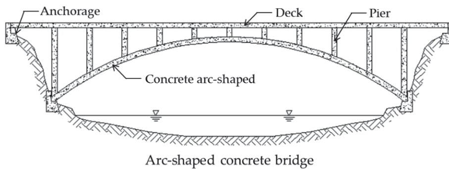
Figure 17. Concrete bridges for medium span lengths.
